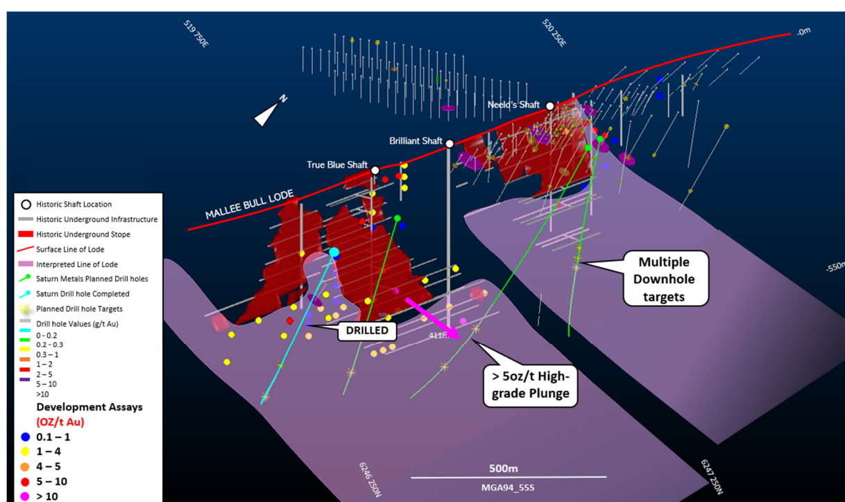
Figure 7 – 3D Representation of planned and completed drill holes relative to old workings, key mineralisation plunges and very high-grade historic face sample data diagram adapted from references as fully outlined in Saturn ASX Announcement dated 21 June 2021.
