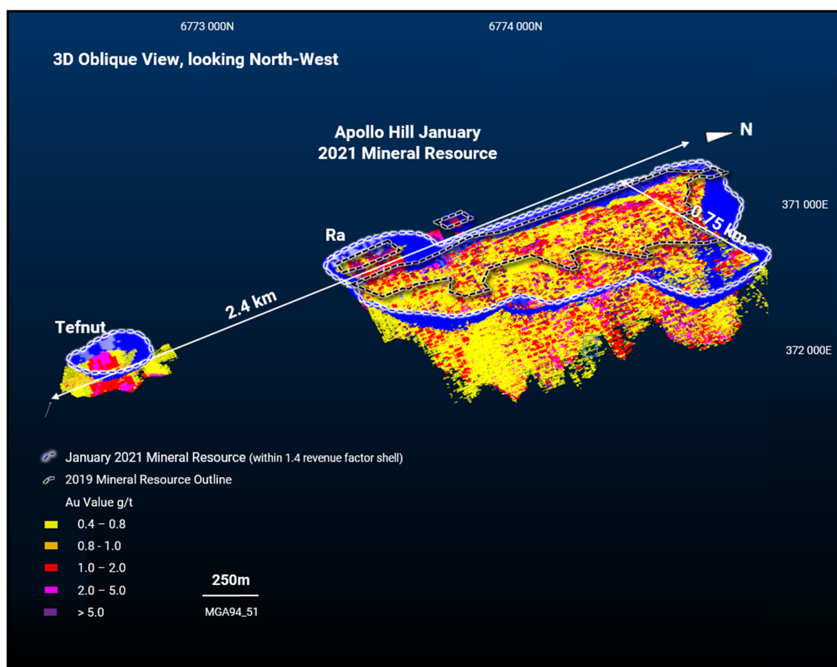
Figure 2 – 3D Representation of the January 2021 Apollo Hill Mineral Resource model and selected pit shell; view looking NW highlights width and robust nature of mineralisation.
