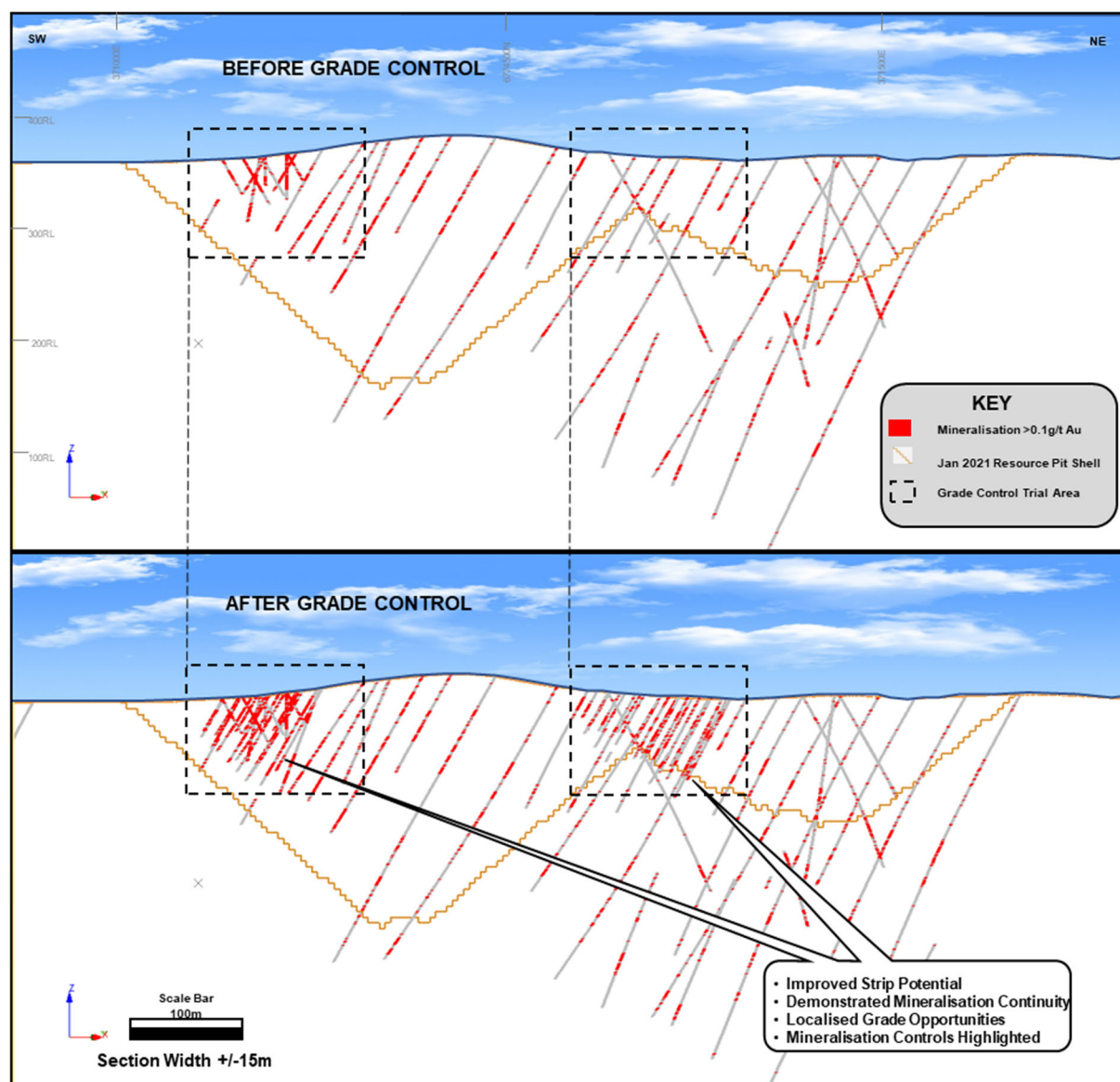
Figure 4 – Mineralisation cross section – before and after trial grade control/ drill density program.
