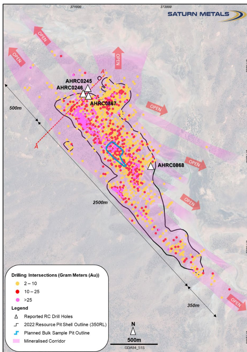
Figure 1 – Plan view of gram metre intersections in context of the Resource Pit Shell, planned bulk sample pit, reported drillhole collar points and section line
