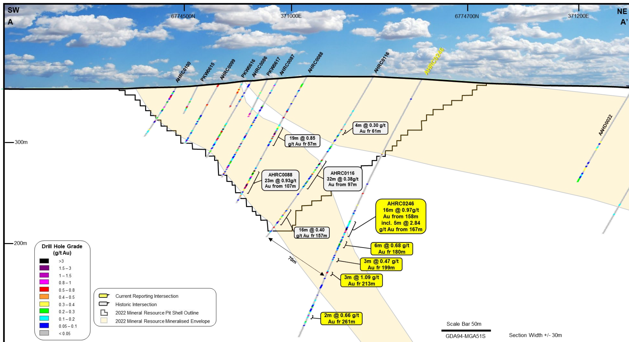
Figure 3 – Simplified geological cross section of AHRC0246 (re-entry extension) relative to historical drilling and the Apollo Hill Mineral Resource Pit Shell.
