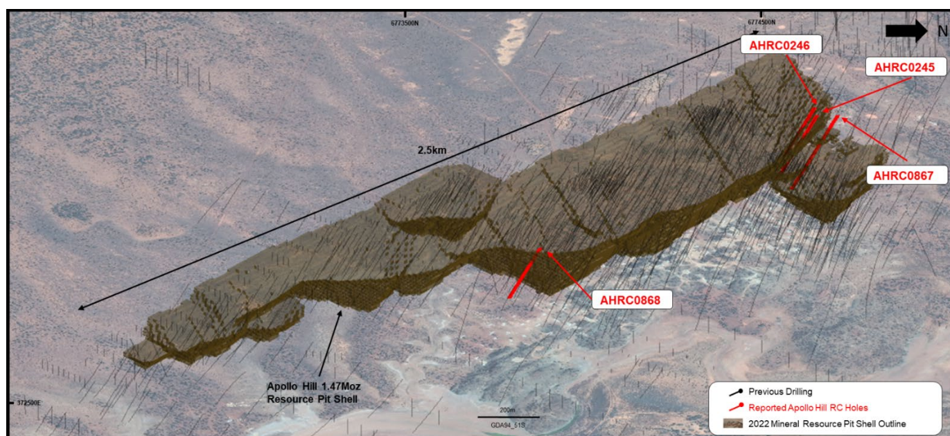
Figure 2 – Oblique view of the Resource Pit Shell, historical and reported drillhole traces.
