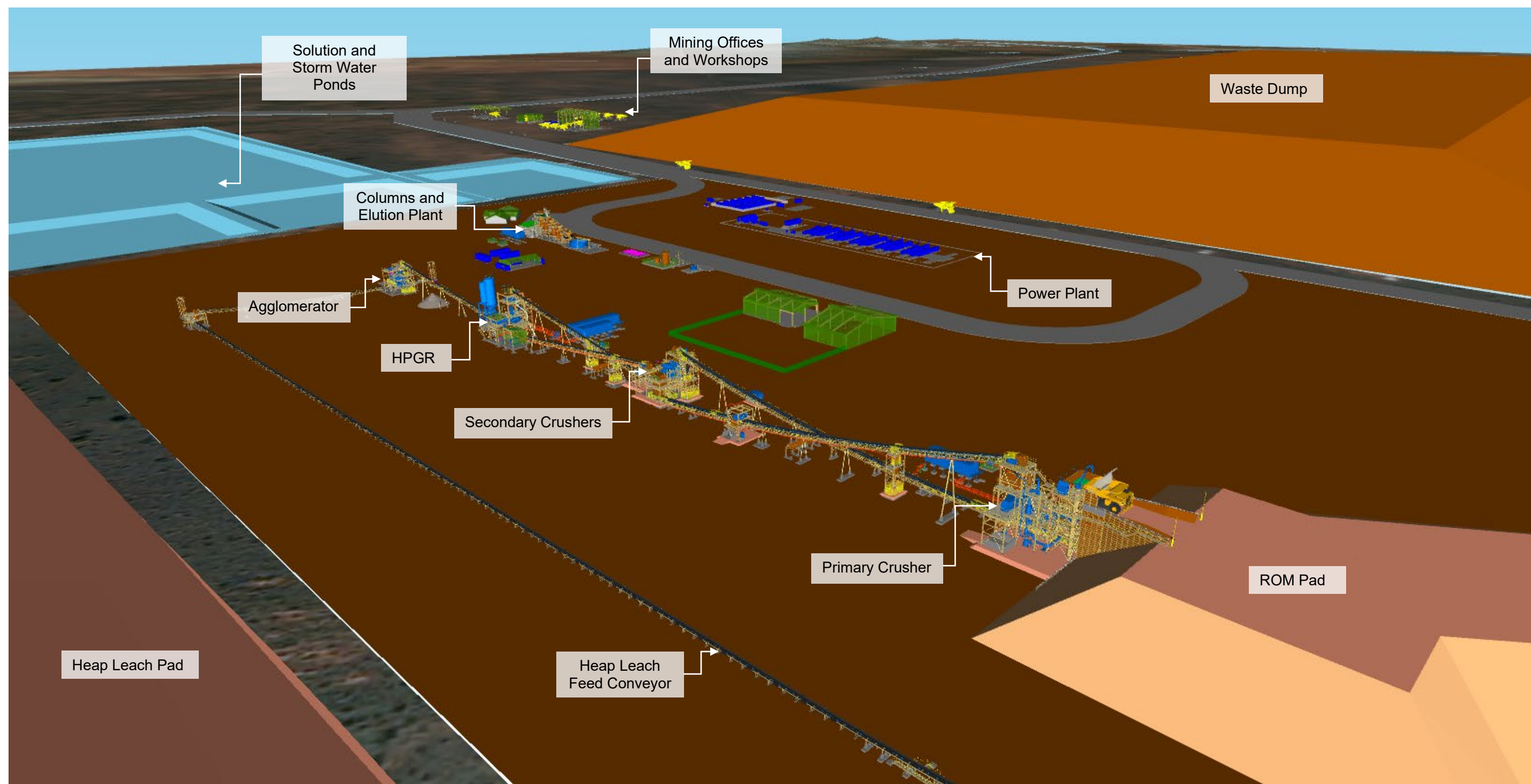
Figure 14 – Conceptual general arrangement – 3D site layout and processing plant.
