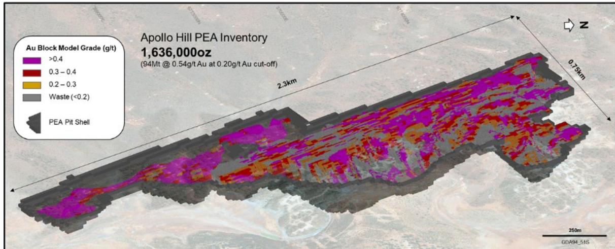
Figure 15 – PEA pit shell and ore and waste blocks by grade.
