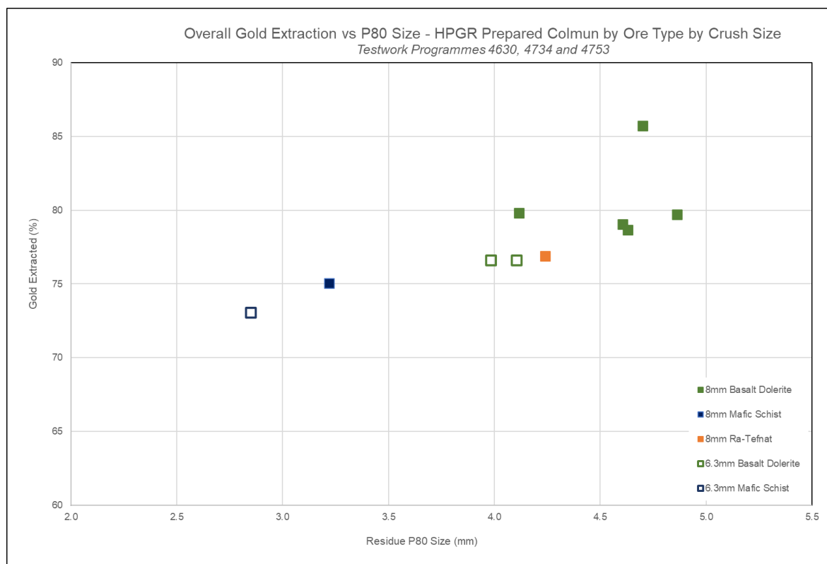
Figure 9 – Average makeup of overall gold extraction by Apollo Hill's main fresh rock types at various P_{80} HPGR crush sizes.
