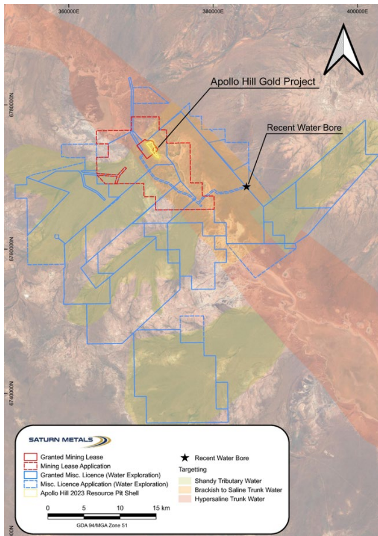
Figure 21 – Saturn Metals water exploration targets, water exploration miscellaneous license and other miscellaneous licenses at Apollo Hill.
