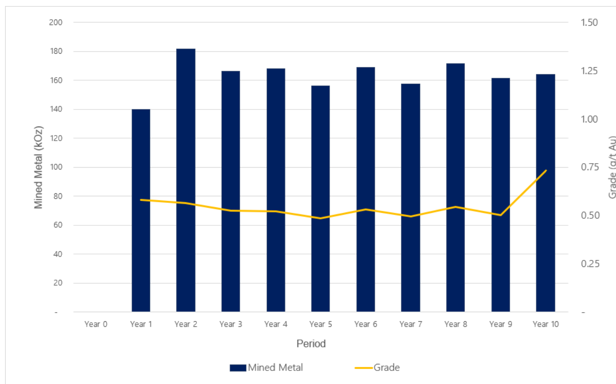
Figure 17 – Open pit annualised ounce production and grade.
