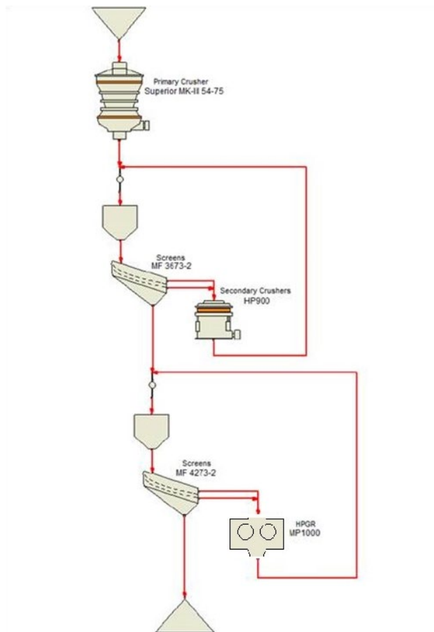
Figure 12 – Detailed crushing flow sheet.
