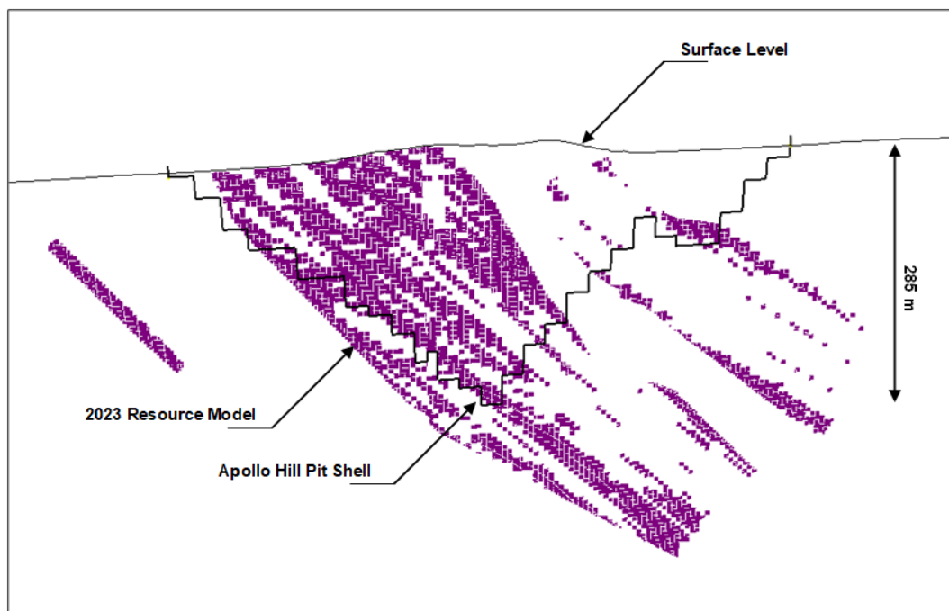
Figure 16 – Section showing PEA pit outline with 2023 Resource Model (constrained to blocks greater than 0.2 g/t); the diagram illustrates large ore mining widths, a low strip ratio and ore material outcropping at surface.
