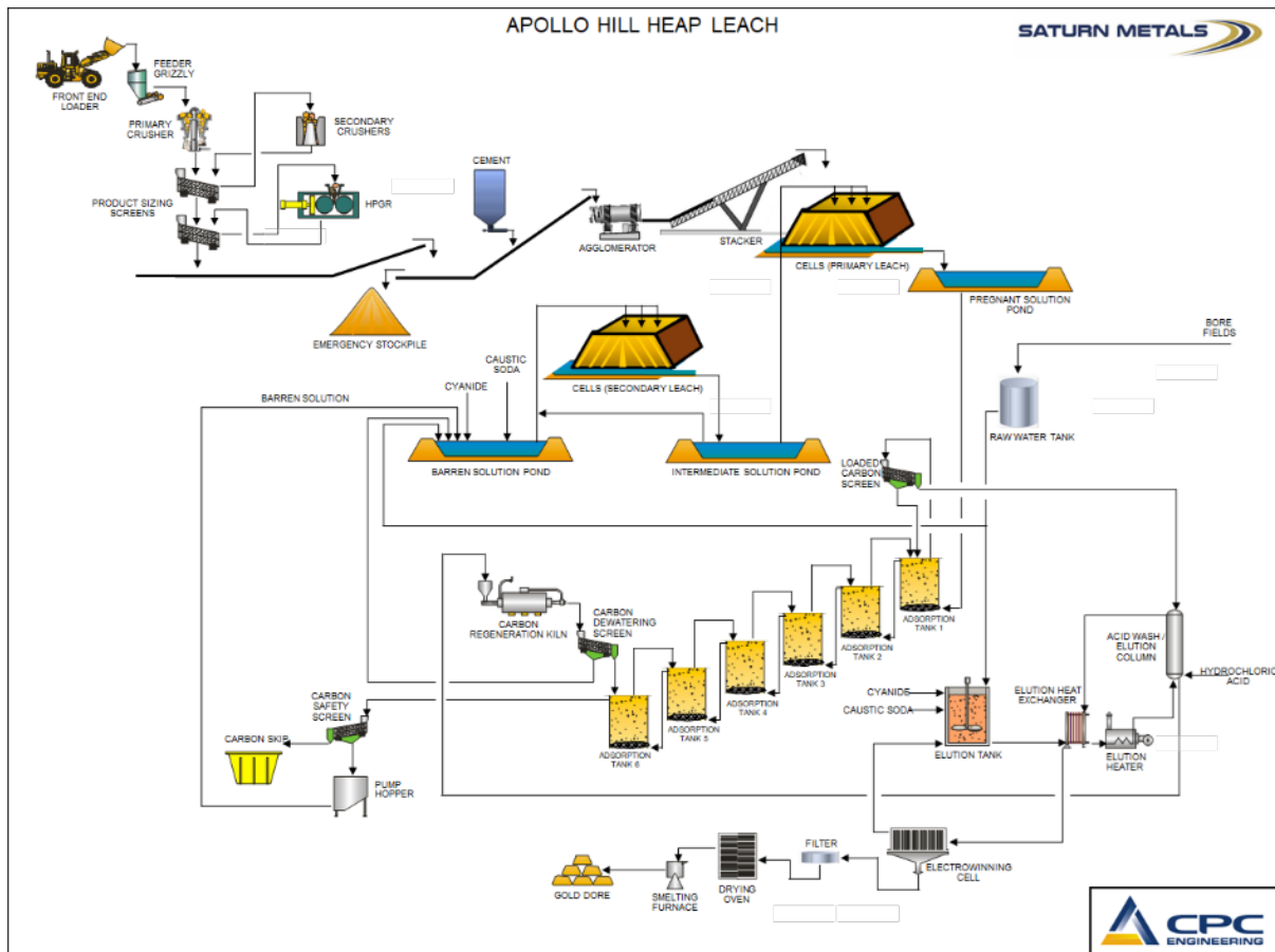
Figure 11 – Process diagrammatic flow schematic.
