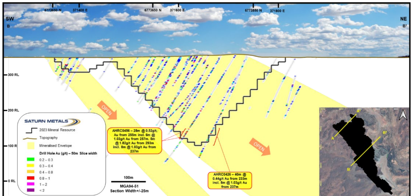
Figure 28 – Apollo Hill Deposit open at depth.
