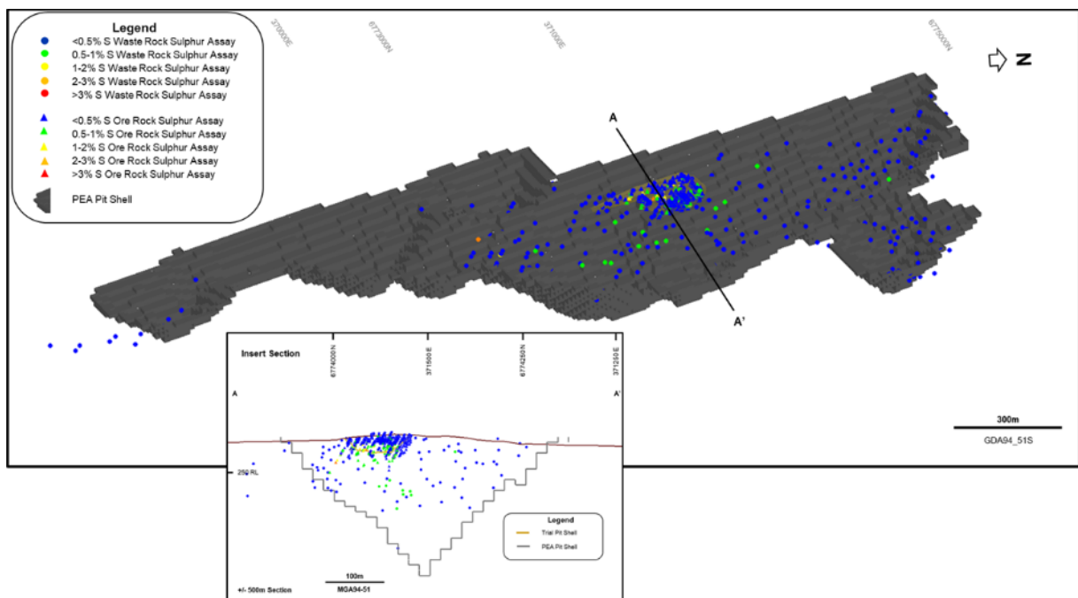
Figure 19 – Open pit sulphur assay locations.
