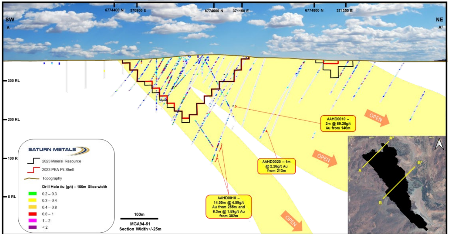
Figure 27 – Apollo Hill Deposit drilled at depth.
