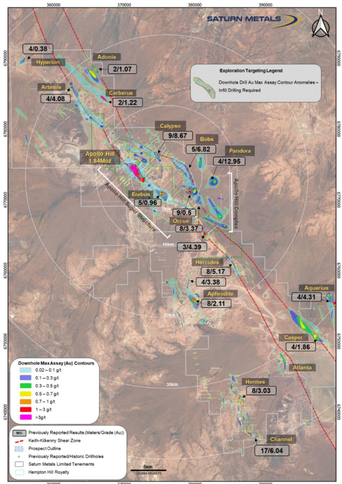
Figure 30 – Apollo Hill regional exploration – prospects, intercepts and targeting.
