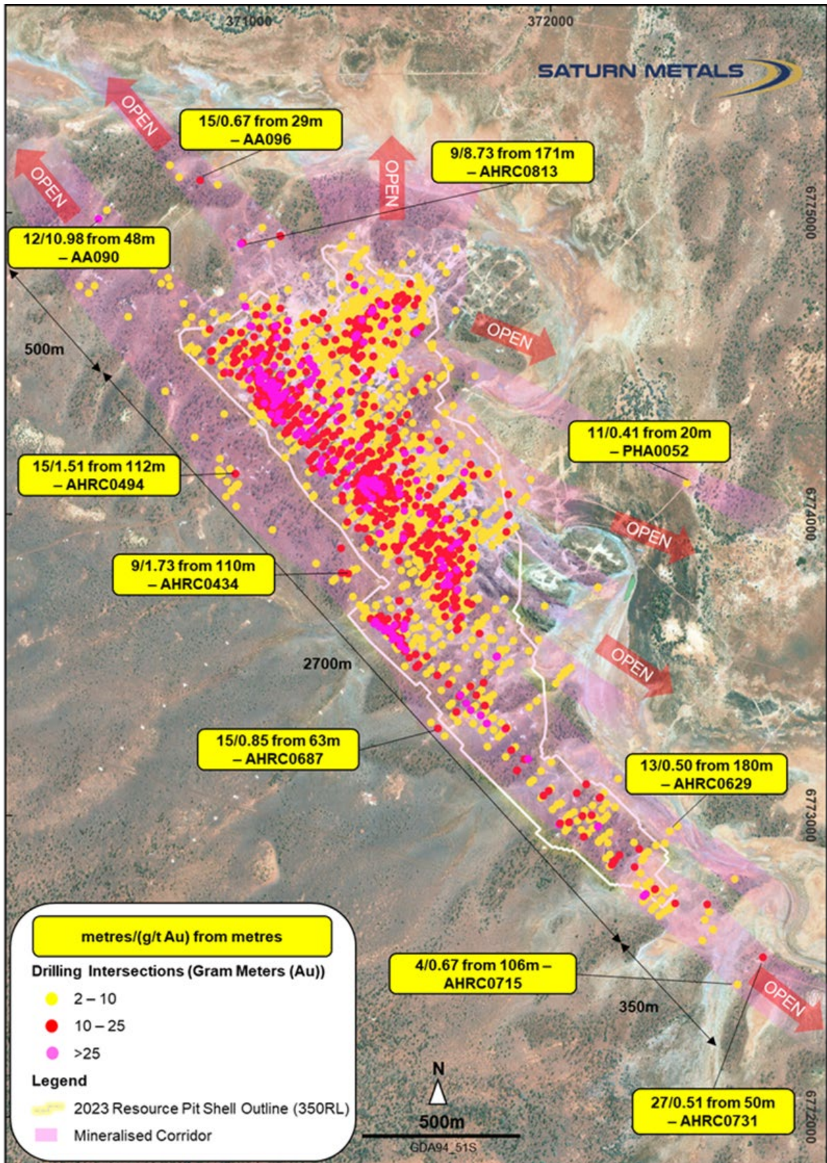
Figure 29 – Strike extension potential at Apollo Hill.
