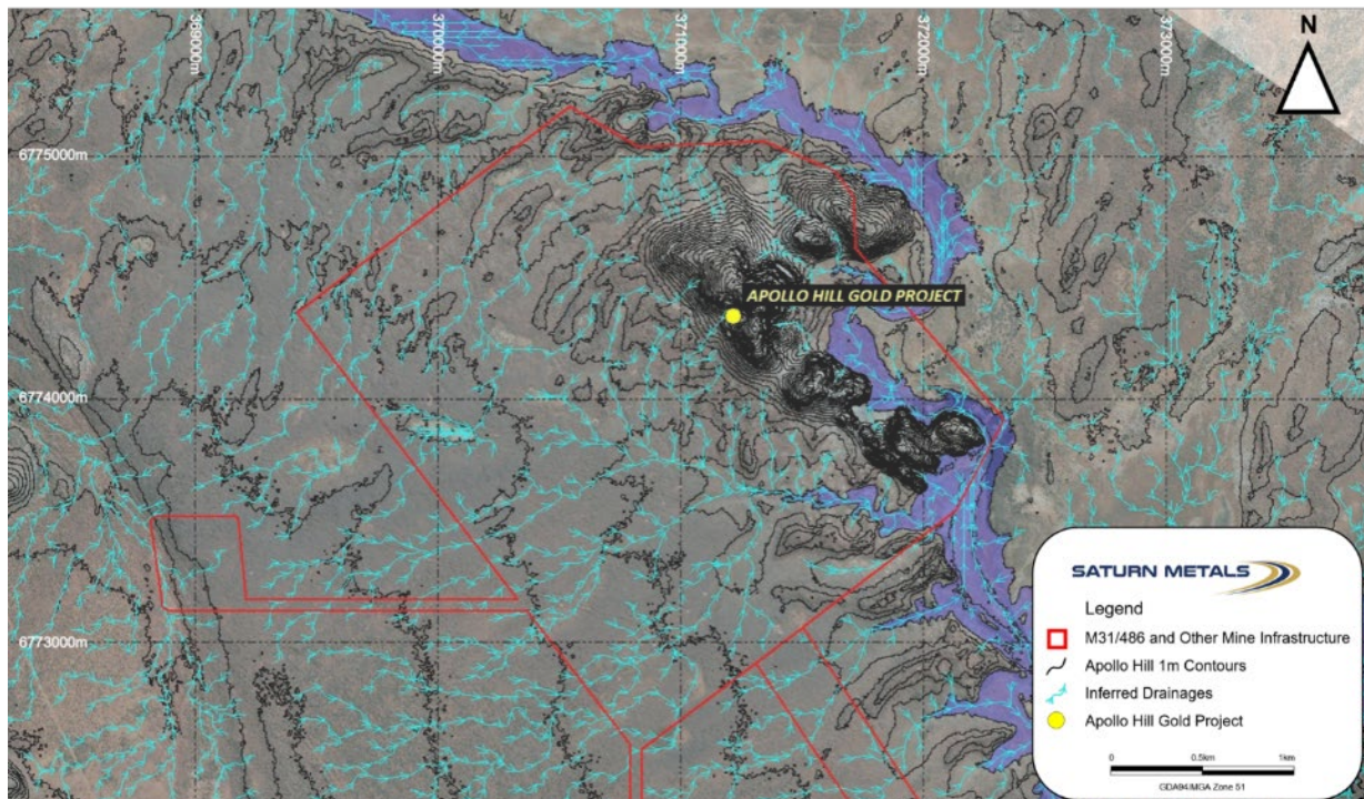
Figure 20 – Inferred drainage channels.
