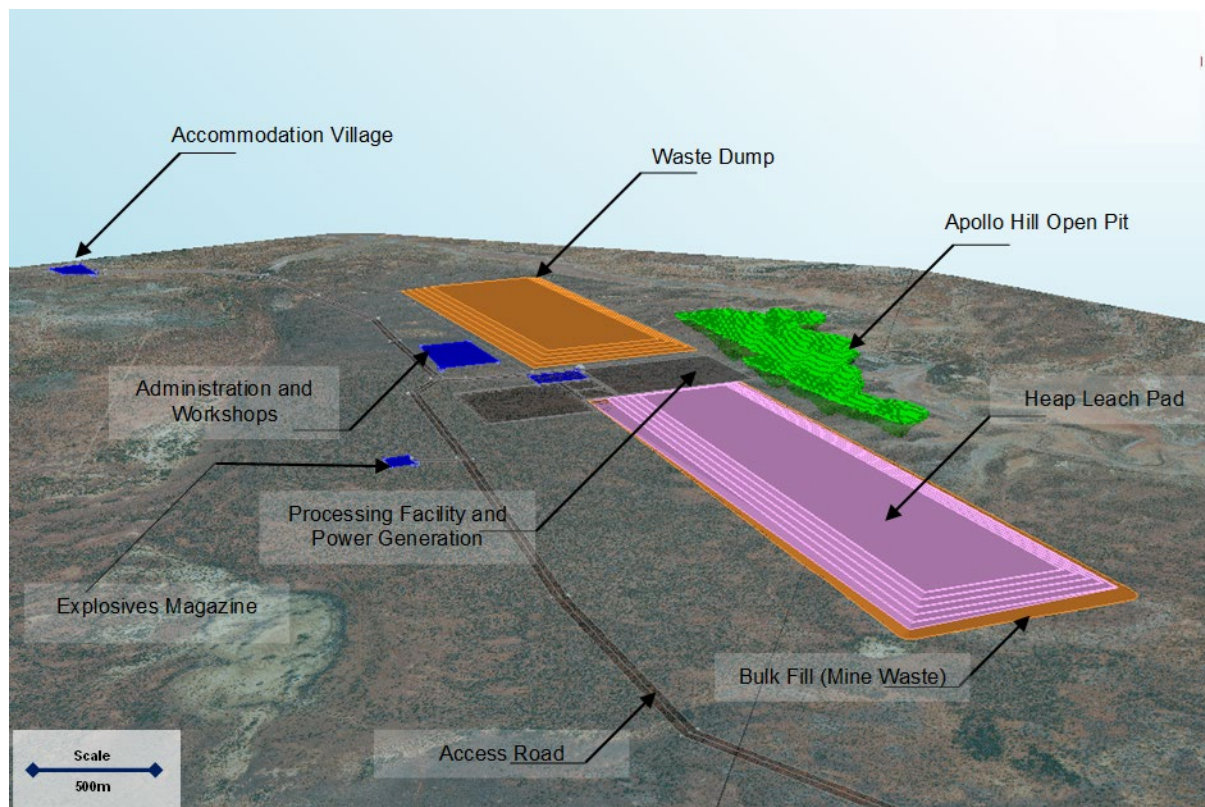
Figure 23 – Apollo Hill planned infrastructure overview, looking North.
