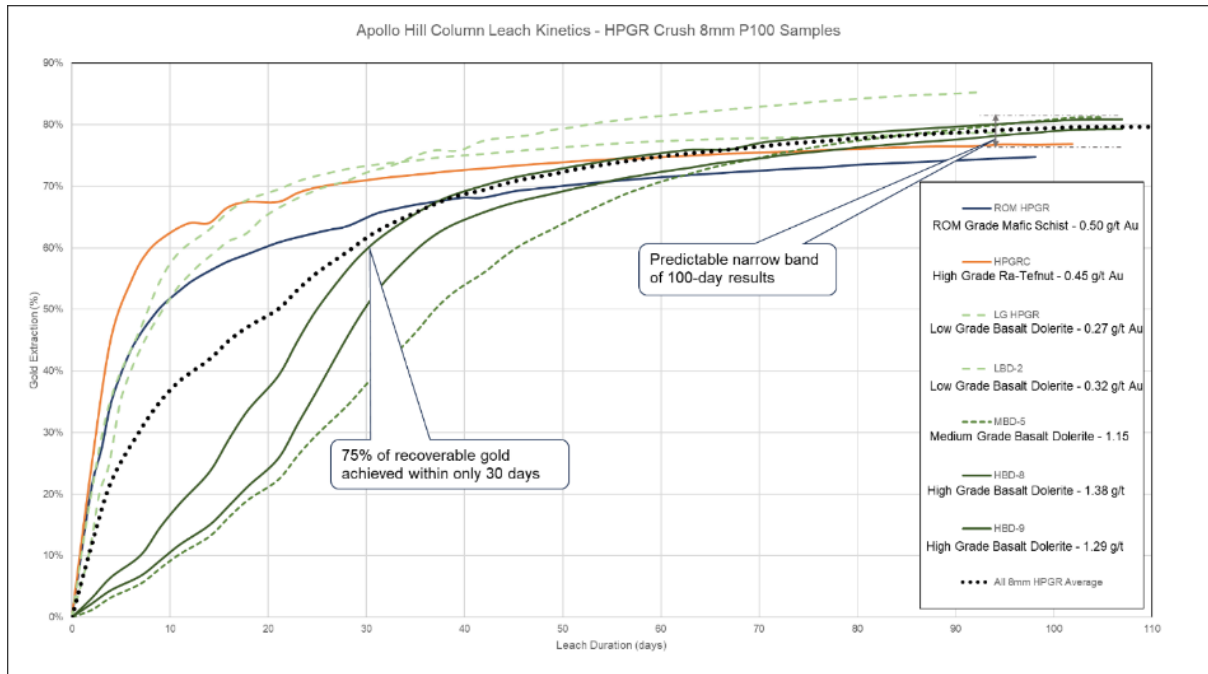
Figure 10 – Recent column leach recovery test curves 8mm HPGR – strong leach kinetics – a predictable narrow band of 100-day recovery results; recovery also illustrated to be insensitive to grade.
