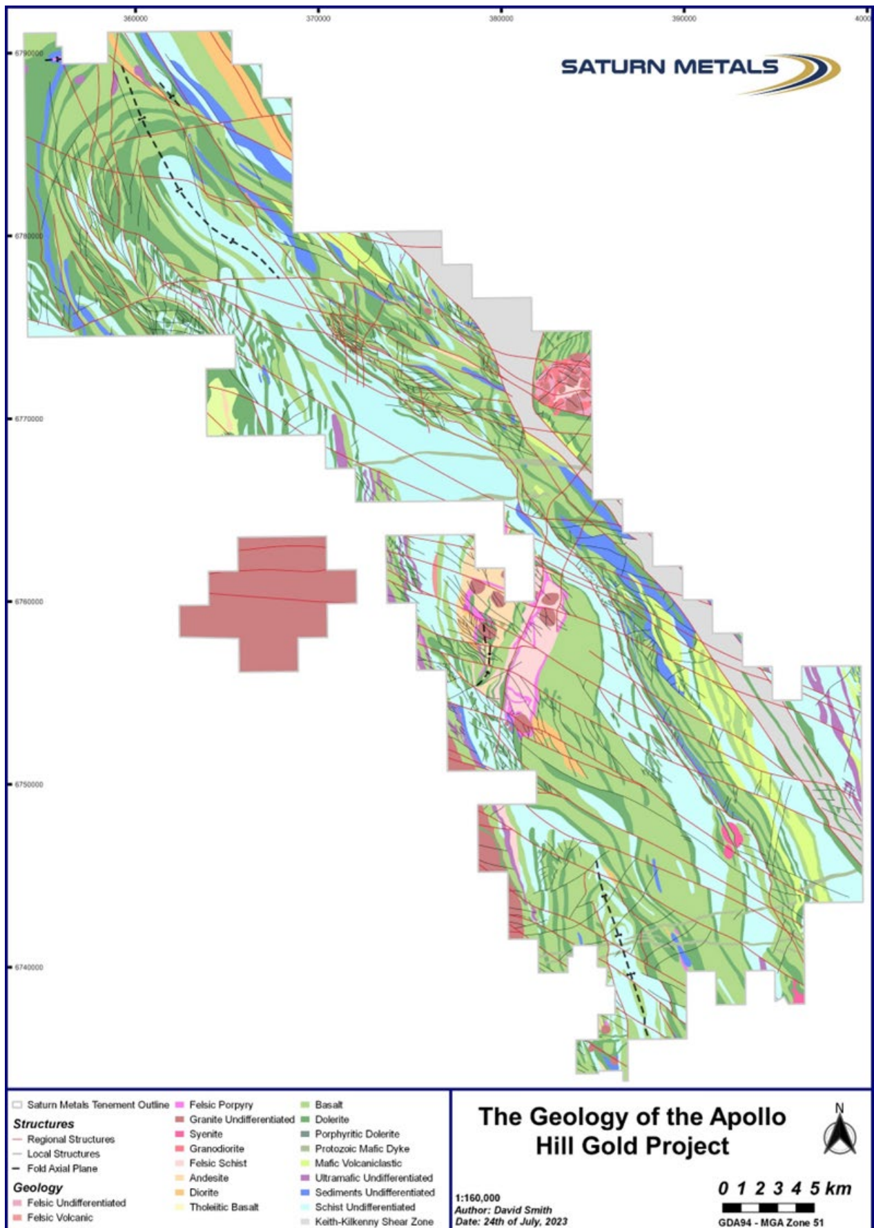
Figure 2 – Saturn Metals Apollo Hill regional geological interpretation.
