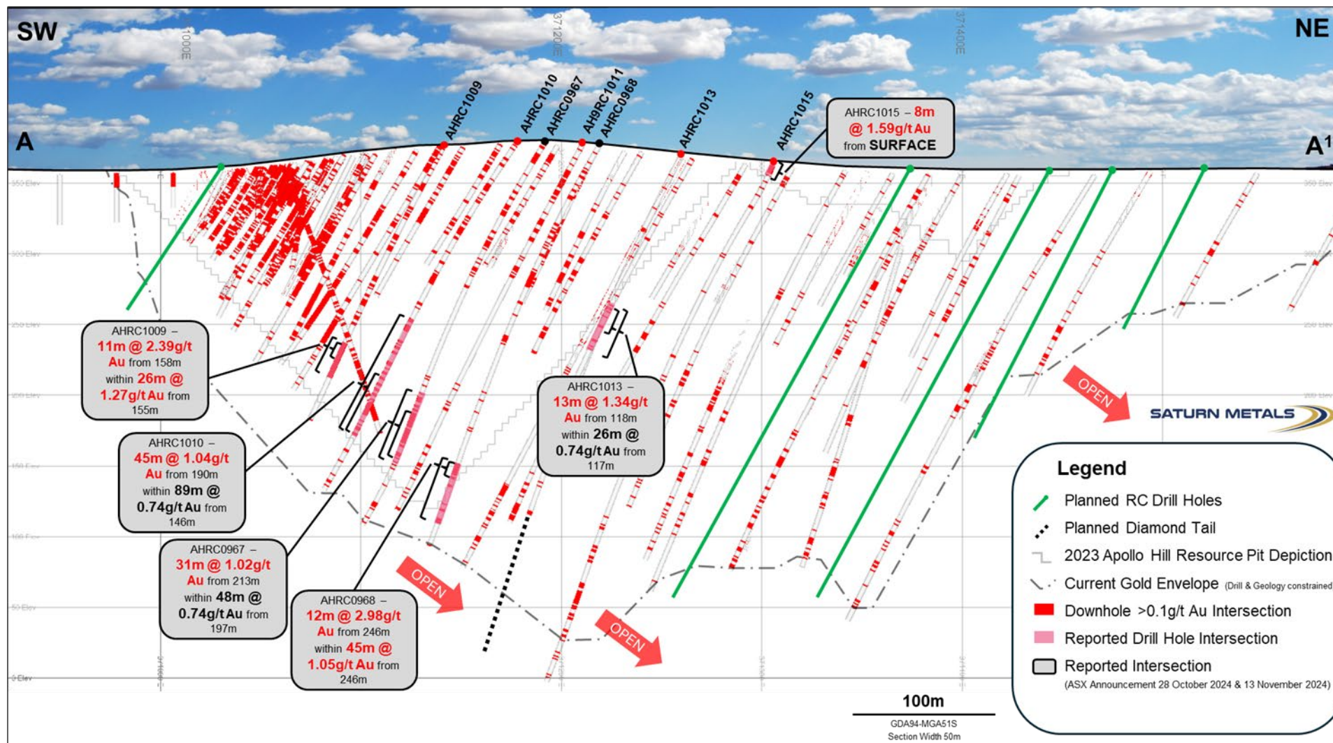
Figure 1 – Simplified geological cross-section showing recent results, mineralisation interpretation, planned RC holes and planned diamond tails; Section location shown in plan on Figure 2 (A-A').
