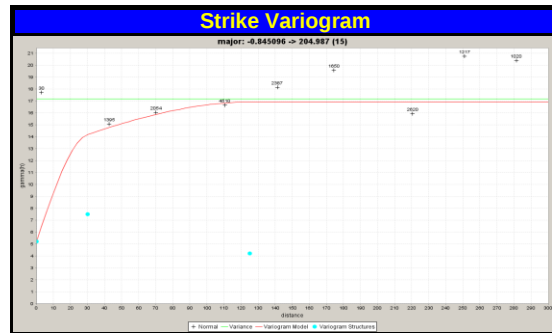
Figure 17.6_1 Los Pumas Project – South Hemisphere Mining Variogram Mn (%) High Grade Domain
