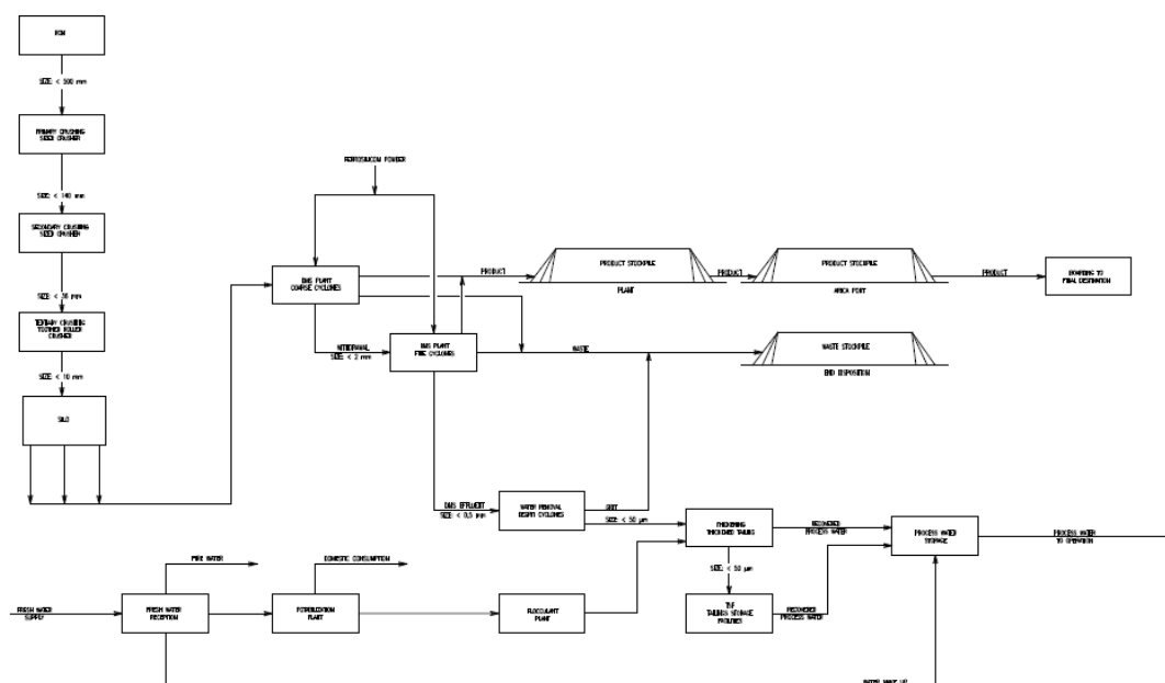
Figure 18.2.1_1 General Process Block Diagram
