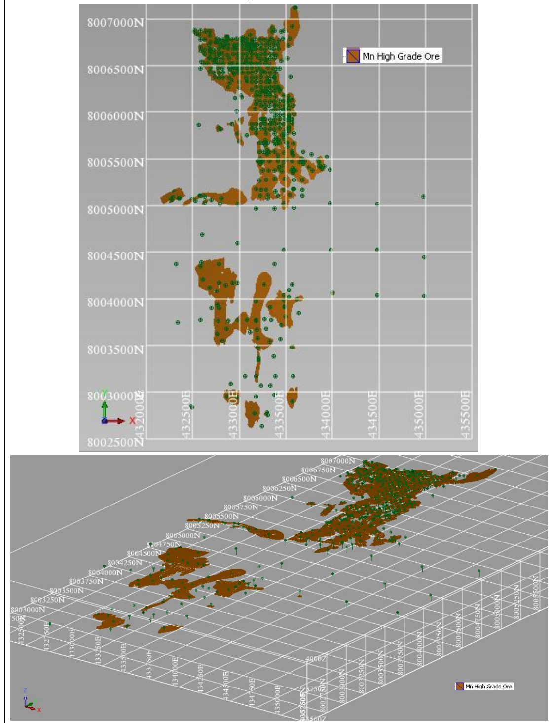
Figure 17.3_5 Los Pumas Project – South Hemisphere Mining 3D High Grade Domain
