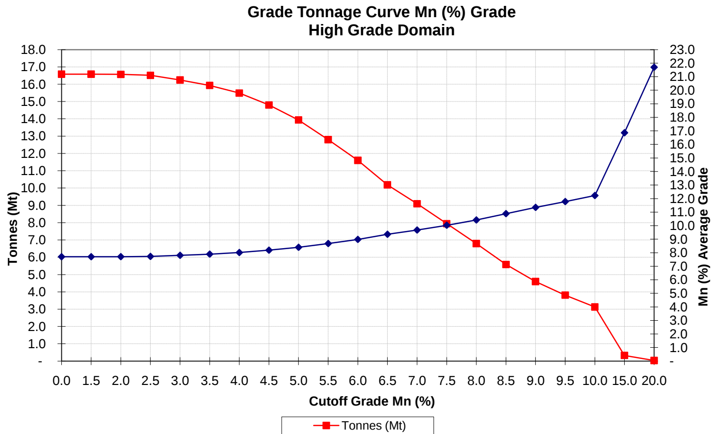
Figure 17.12_1 Los Pumas Project – South Hemisphere Mining Grade x Tonnage Curve– High Grade Domain
