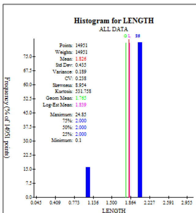
Figure 14.4_1 Sample Length (m) – All Drilling
