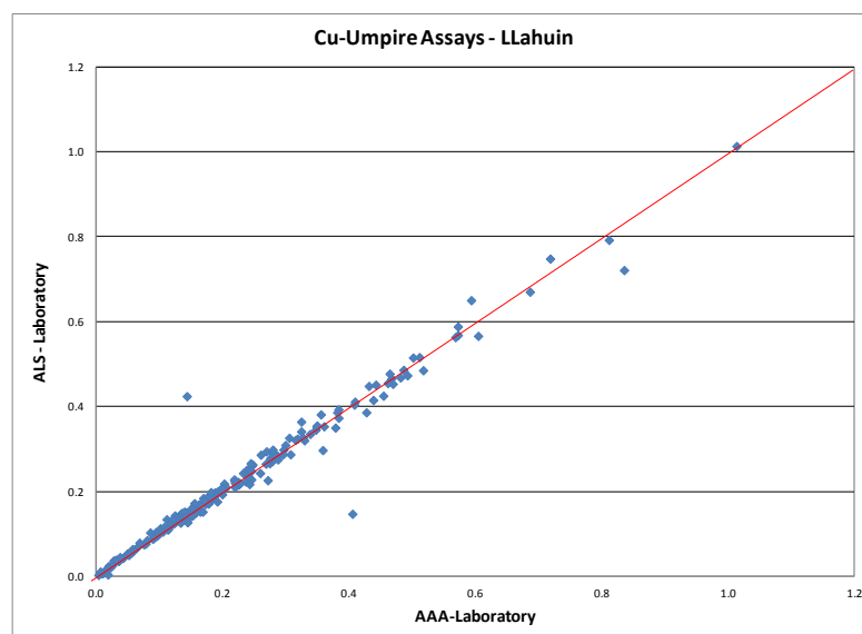
Figure 12.2.3_1 Umpire Assays - Cu
