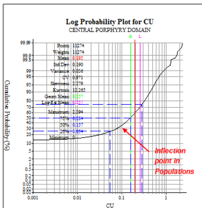
Figure 14.5_1 Log Probability Chart (Cu) – Central Porphyry Zone Composites
