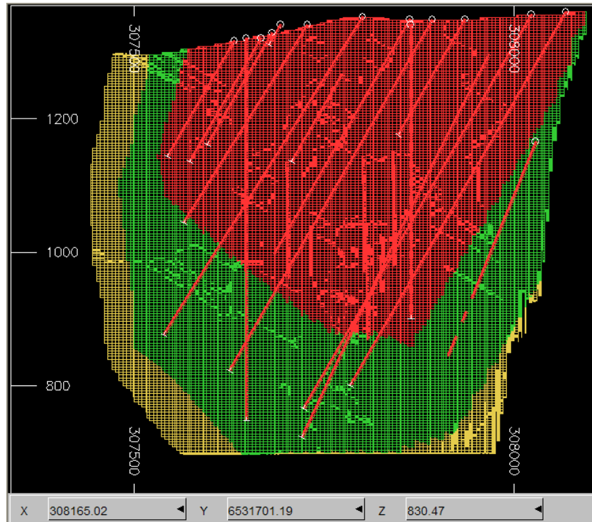
Figure 14.11_1 Central Porphyry Zone - Cross Section – Typical Resource Coding
