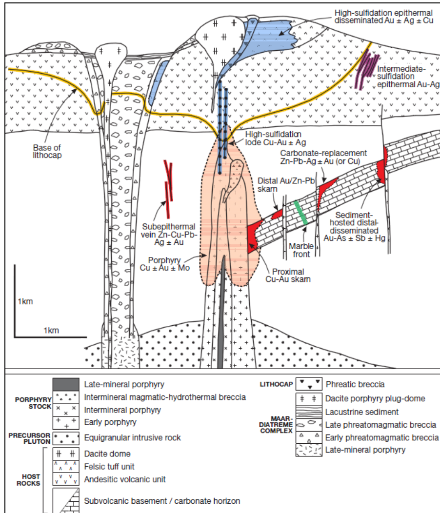
Figure 8_1 Genetic Model for Porphyry Copper Deposits (Sillitoe, 2011)
