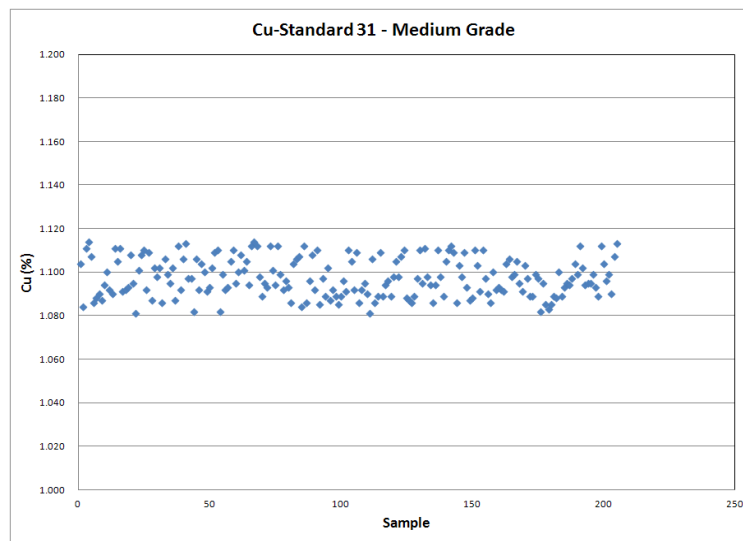
Figure 12.2.3_1 Standards – Medium Grade Cu
