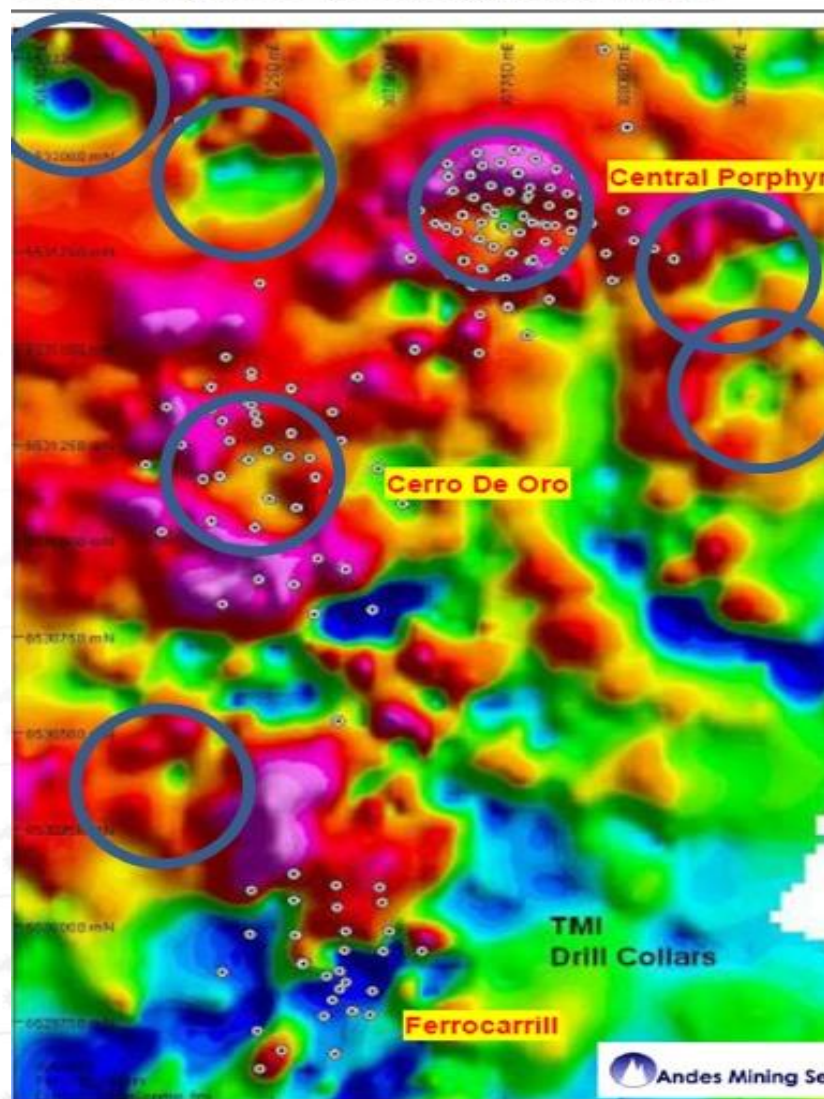
Total Magnetic Intensity (TMI) Maps
