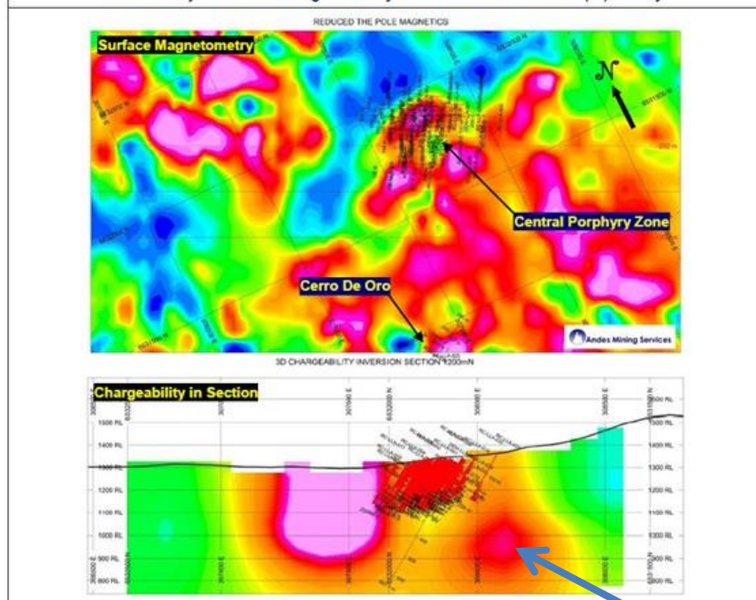
Llahuin Project - Surface Magnetometry and Induced Polarization (IP) Survey
