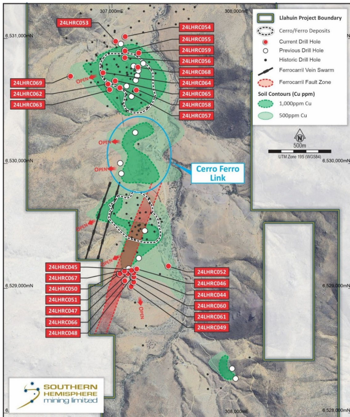
Figure 13. – Location Map showing the Llahuin Cerro and Ferro and Ferro South Zones 2024 drilling in red, 2023 drilling in white, prior drill collars in black, and geochemistry.
