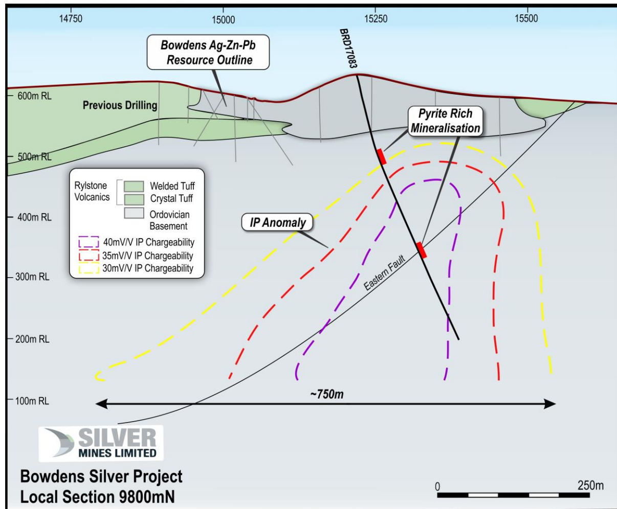
Figure 3. Cross Section of BRD17083.
