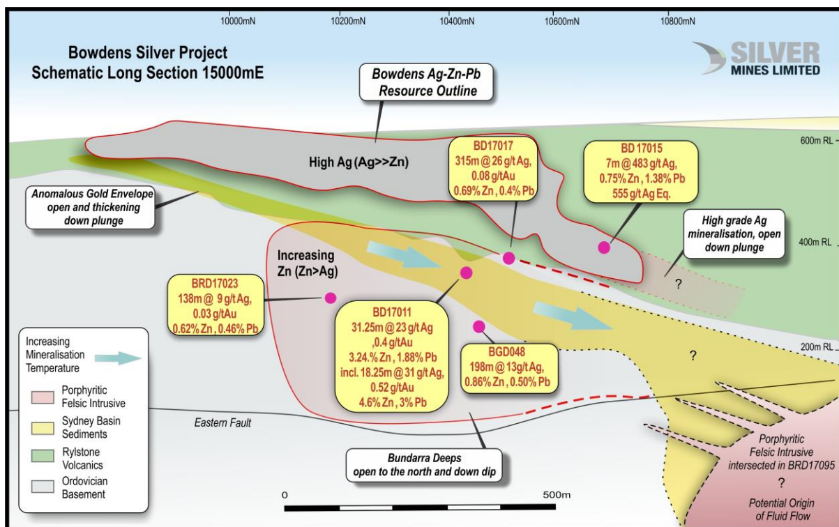
Figure 3. Schematic Long Section highlighting the Bowdens Resource and the northwest exploration target area.
