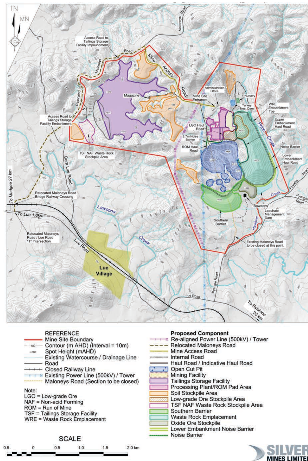
Figure 4: Bowdens Silver Preliminary Mine Site Layout.
