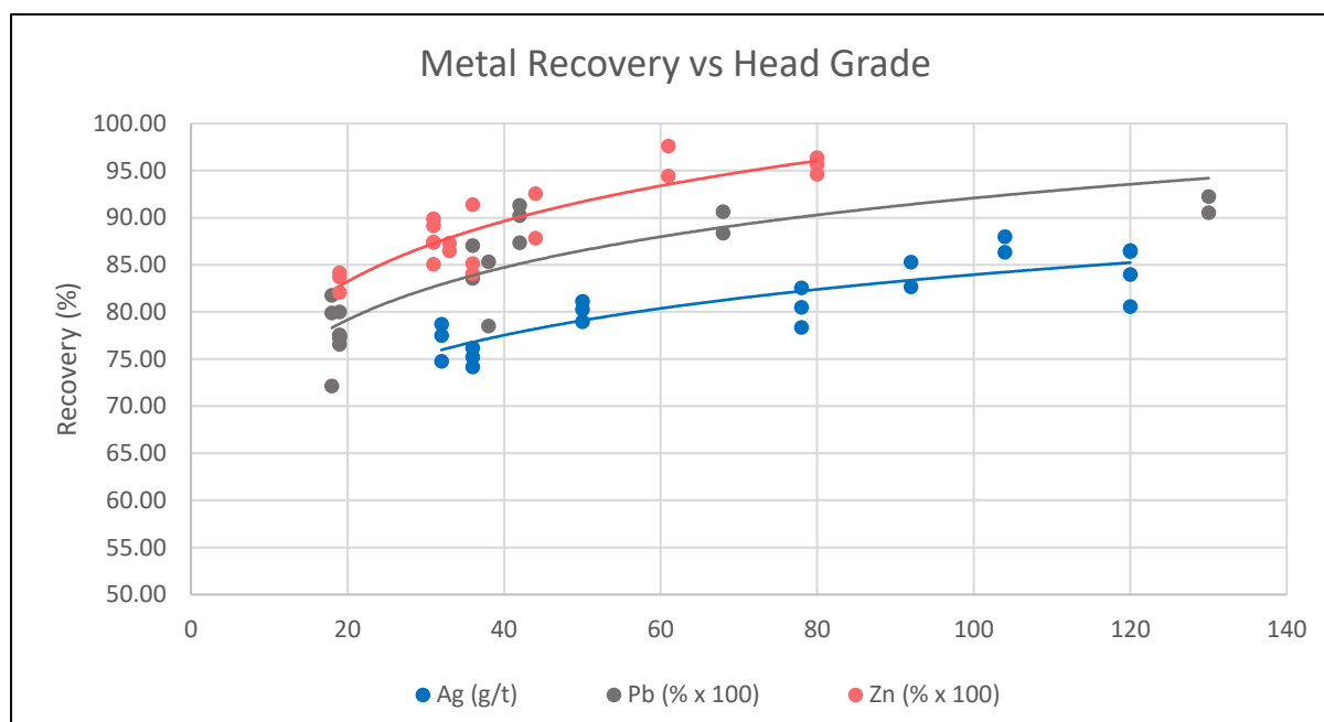
Figure 2 – Recovery versus Head Grade
