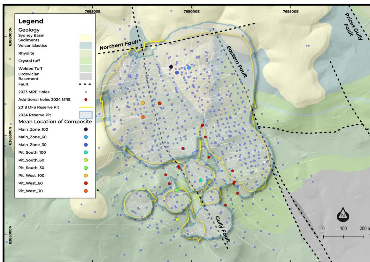
Figure 3 - Location of additional drilling for the 2024 MRE, and changes in Reserve pit designs
