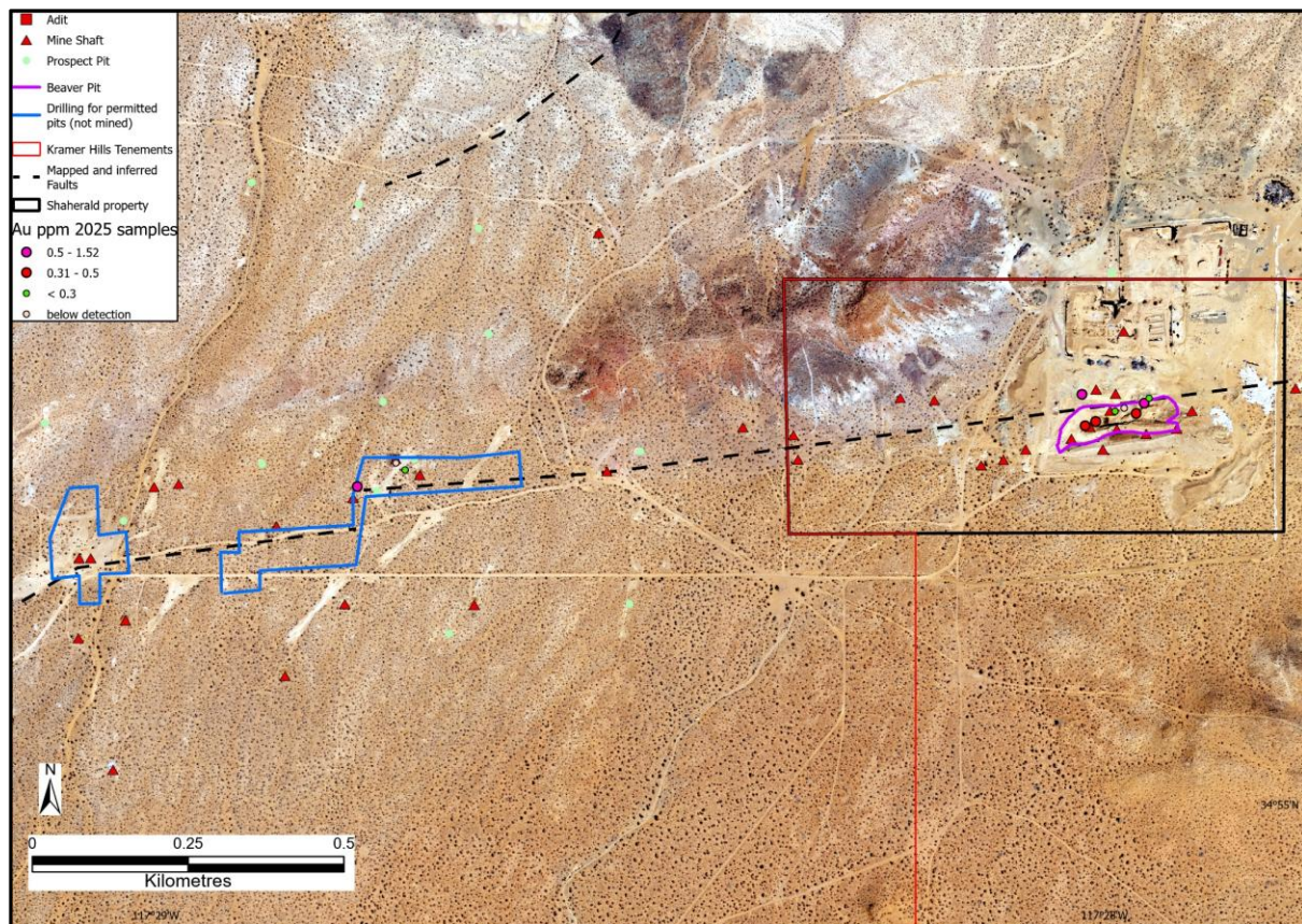
Figure 5: Zoomed view of the Exploration Target area, covering the Shaherald Pit and 1980's drilling areas that resulted in permitted open-pits that were not mined. Note alignment with a mapped fault zone and presence of mine shafts that are spread along the zone, which were all worked prior to 1942. Silver Mines verification samples taken in 2025, with results up to 1.5g/t gold, confirm presence of mineralised system.
