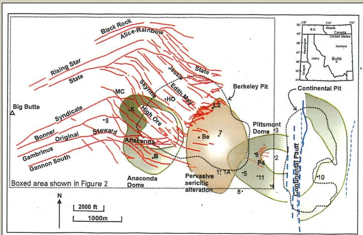
Figure 10. Schematic plan of Butte, Montana showing the distribution of the extensive lode-style copper mineralised veins and the surface projections of the Anaconda and Pittsmond Domes (read porphyries). Figure provided by Dr Greg Corbett.
