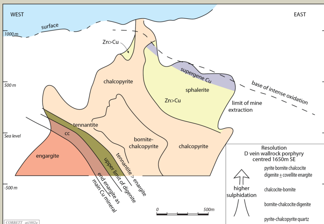
Figure 9. Schematic long section of the Magma Mine veins showing the zonation from arsenical copper sulphides at depth typical of a high-sulphidation mineralisation assemblage proximal to the porphyry source (right-side annotation) moving outwards laterally and vertically to a low-sulphidation mineralisation assemblage. Figure provided by Dr Greg Corbett.
