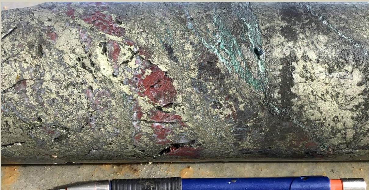
Banded massive pyrite+chalcopyrite, minor quartz+hematite+green clay. 163.9m.
