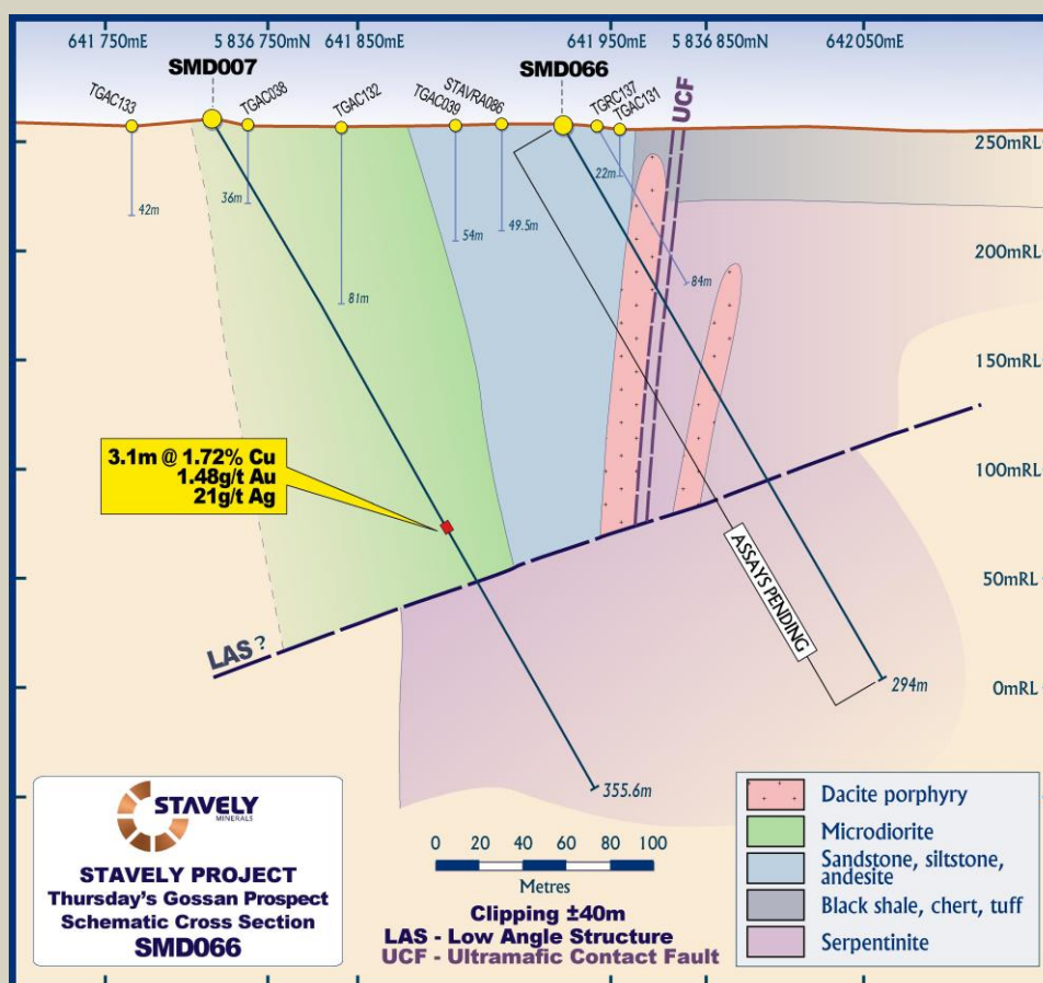
Figure 9. SMD066 drill section.
