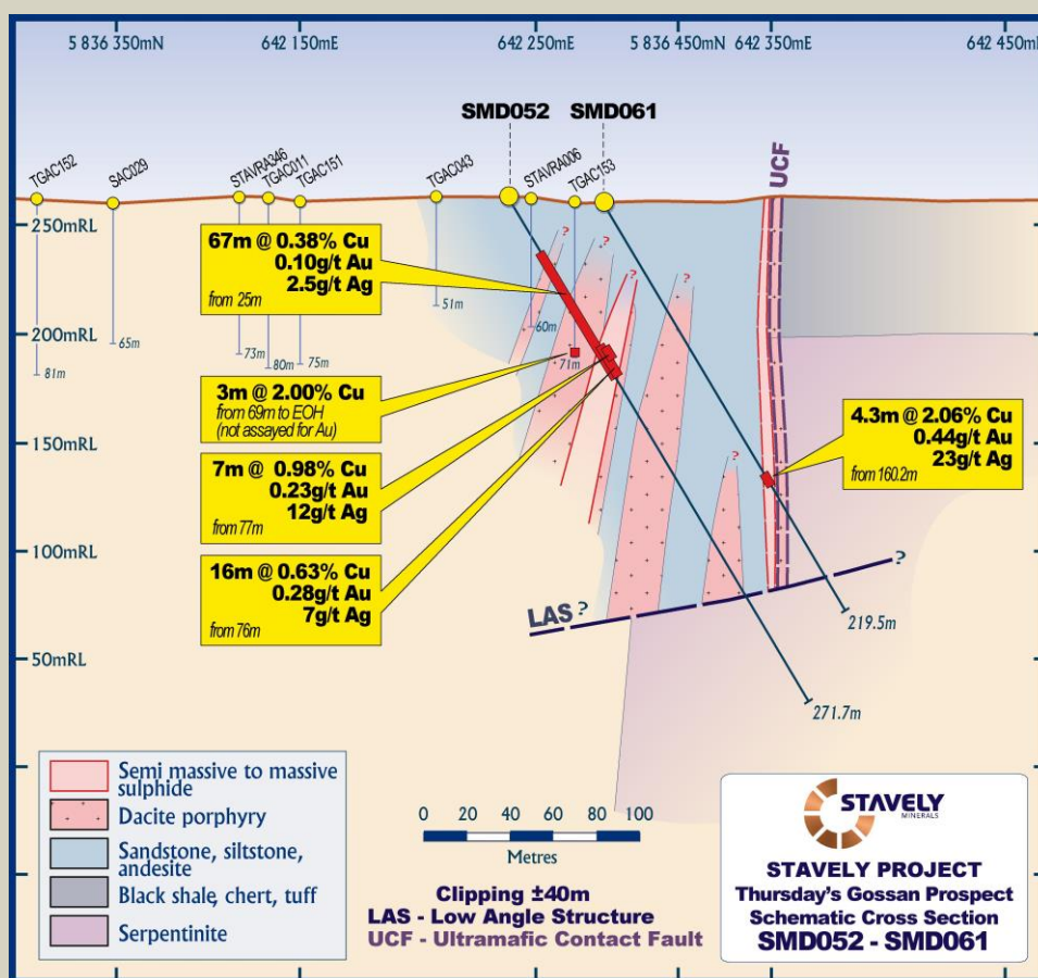
Figure 5. SMD061 drill section.
