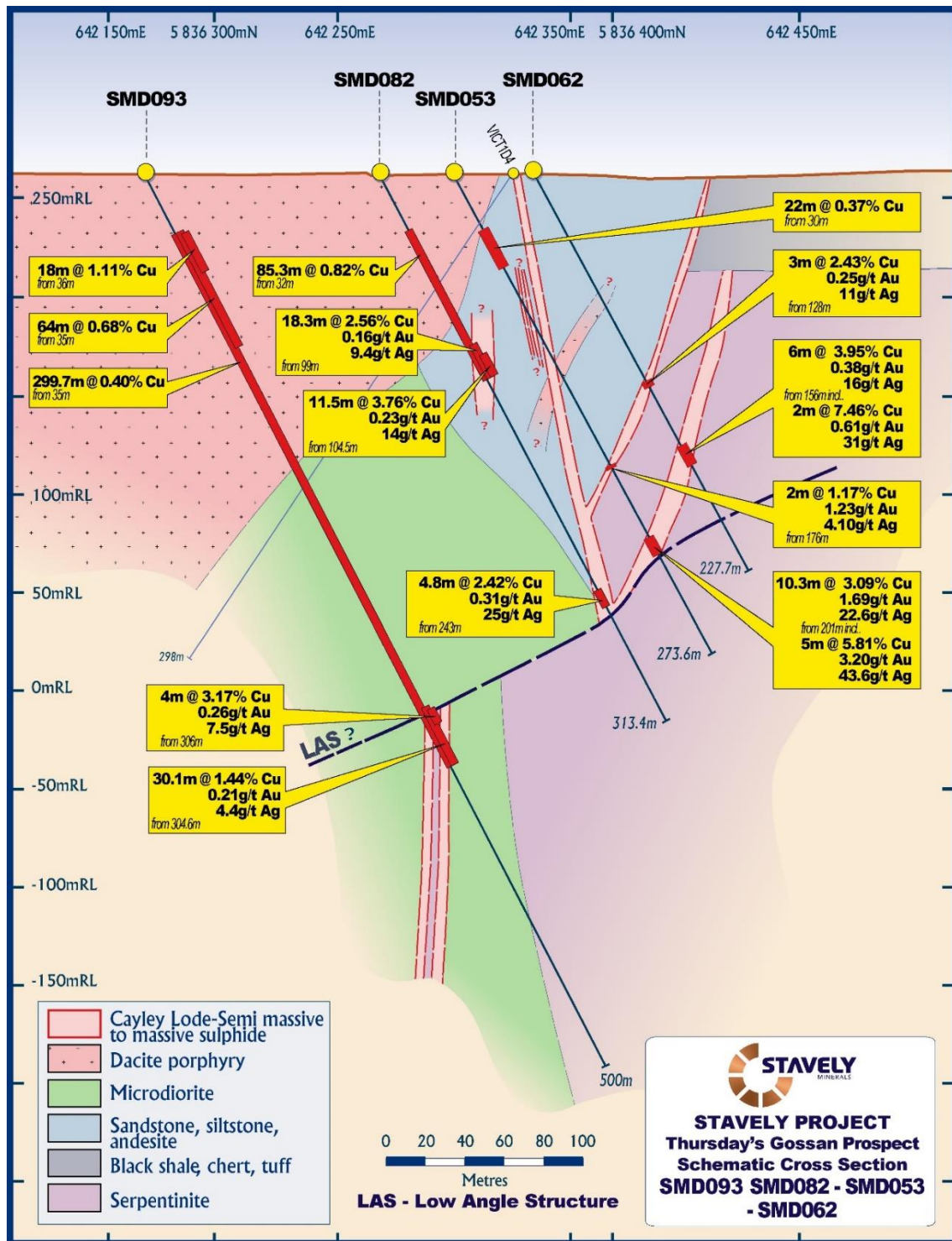
Figure 5. SMD093 drill section.
