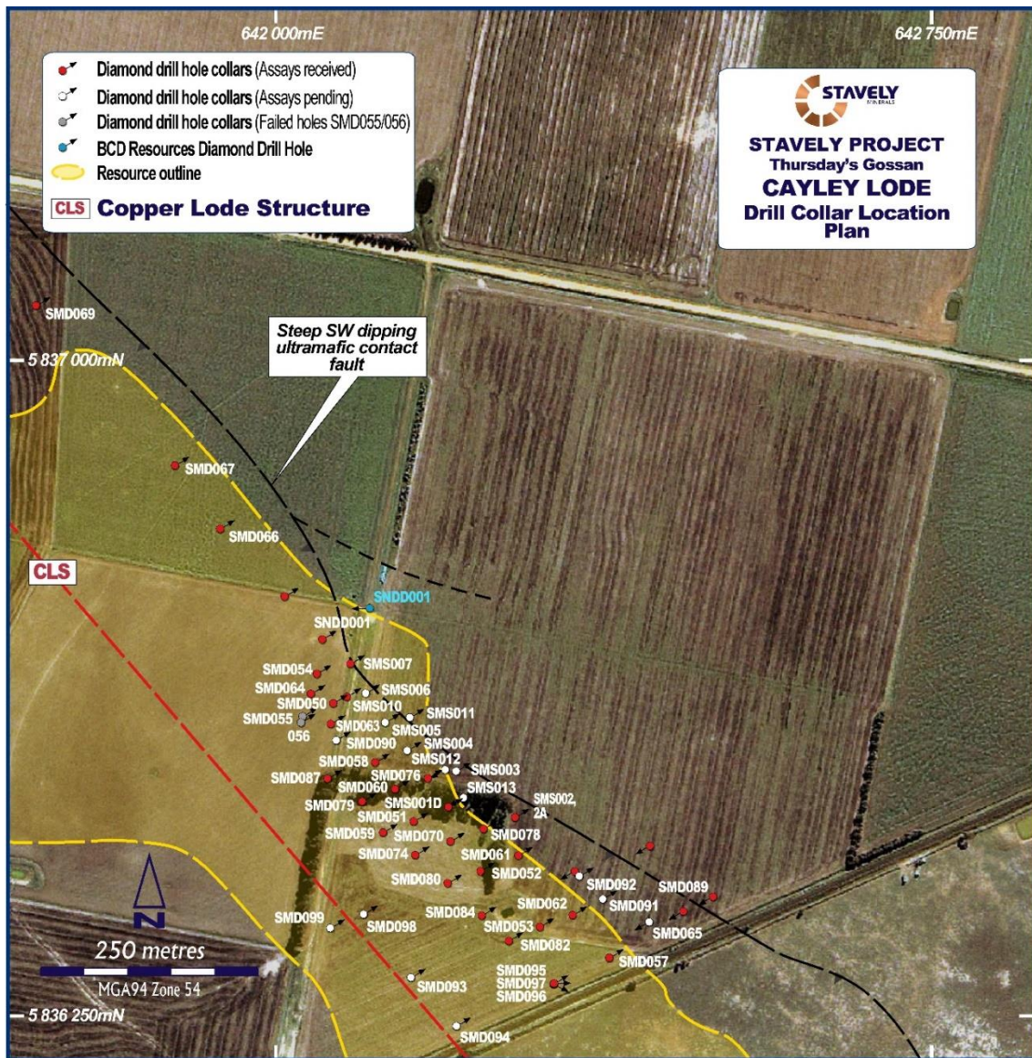
Figure 2. Thursdays Gossan drill collar location plan.
