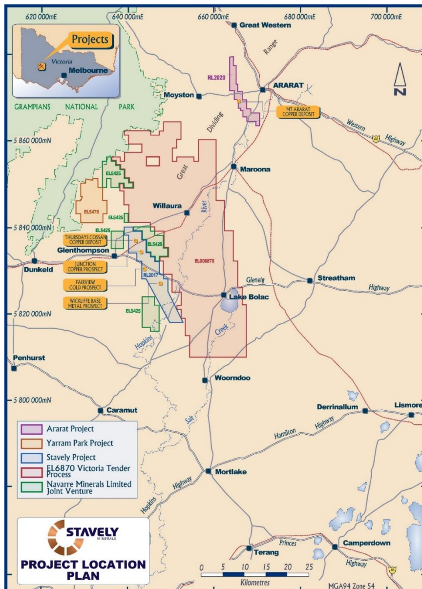
Figure 1. Stavelly Project location map.
