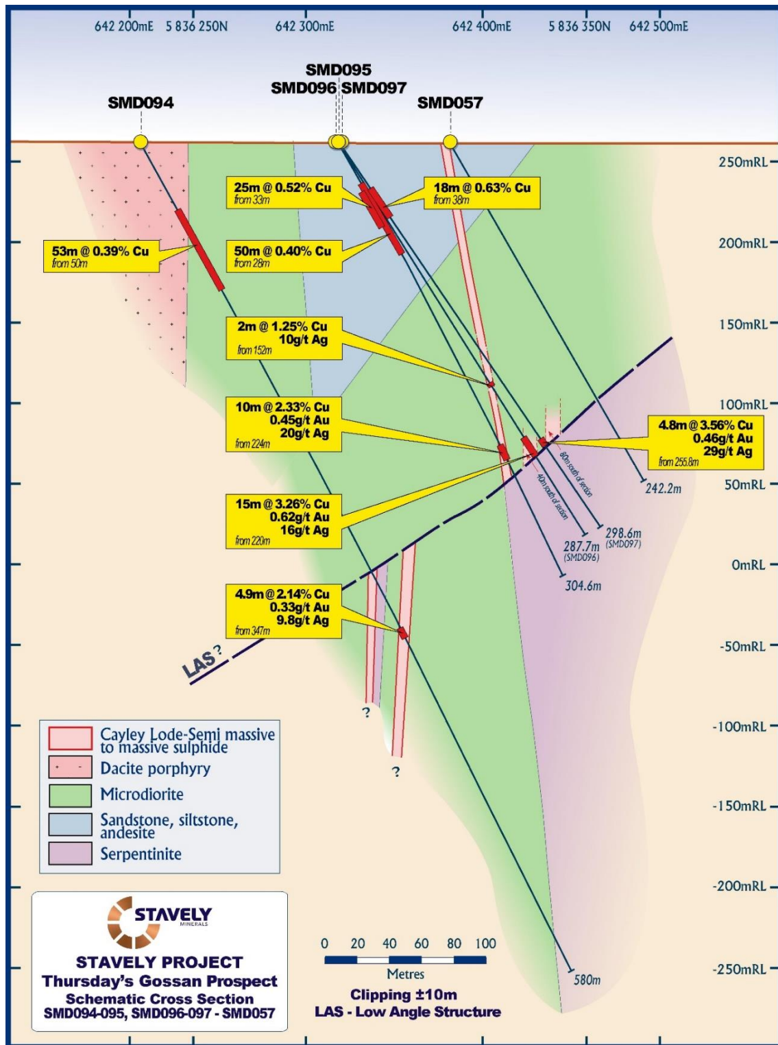
Figure 6. SMD094-97 drill section.
