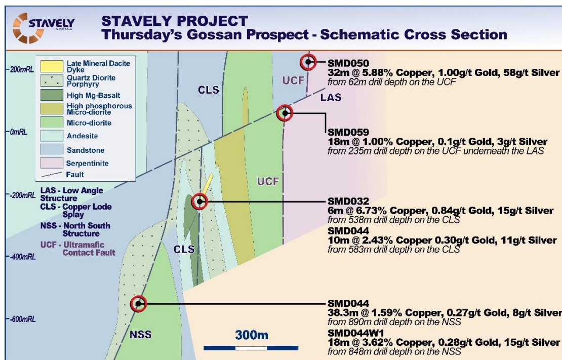
Figure 7. Schematic cross-section of the Thursday's Gossan prospect. Note that the current Cayley Lode Mineral Resource drilling is focused only on the mineralisation located above the LAS on the UCF.
