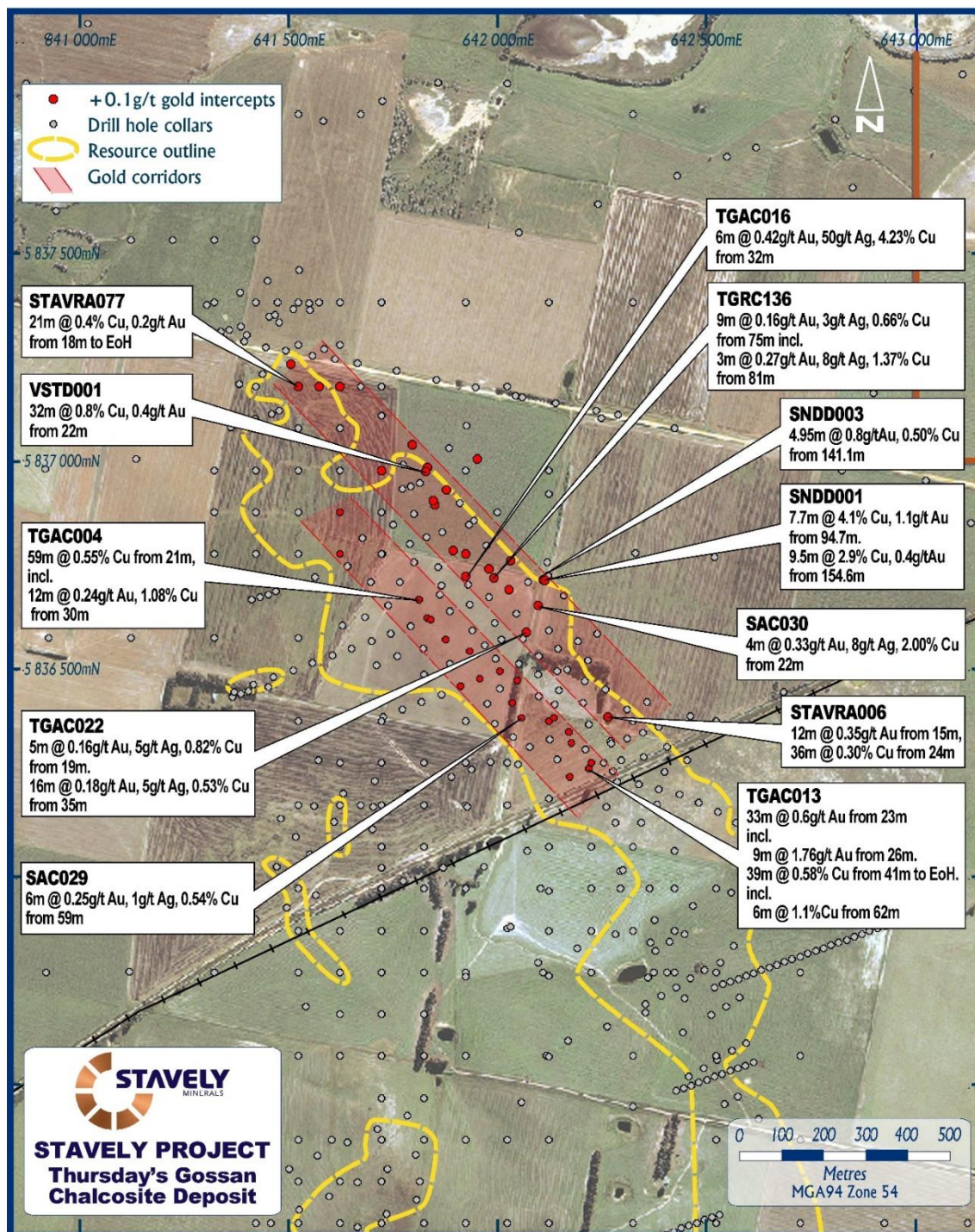
Figure 4. Thursdays Gossan chalcocite-enriched Mineral Resources outline in dashed yellow and the two parallel near-surface zones of higher-grade copper±gold±silver (some drill holes assayed for Cu+Au+Ag, some for only Cu+Au and some for Cu only).
