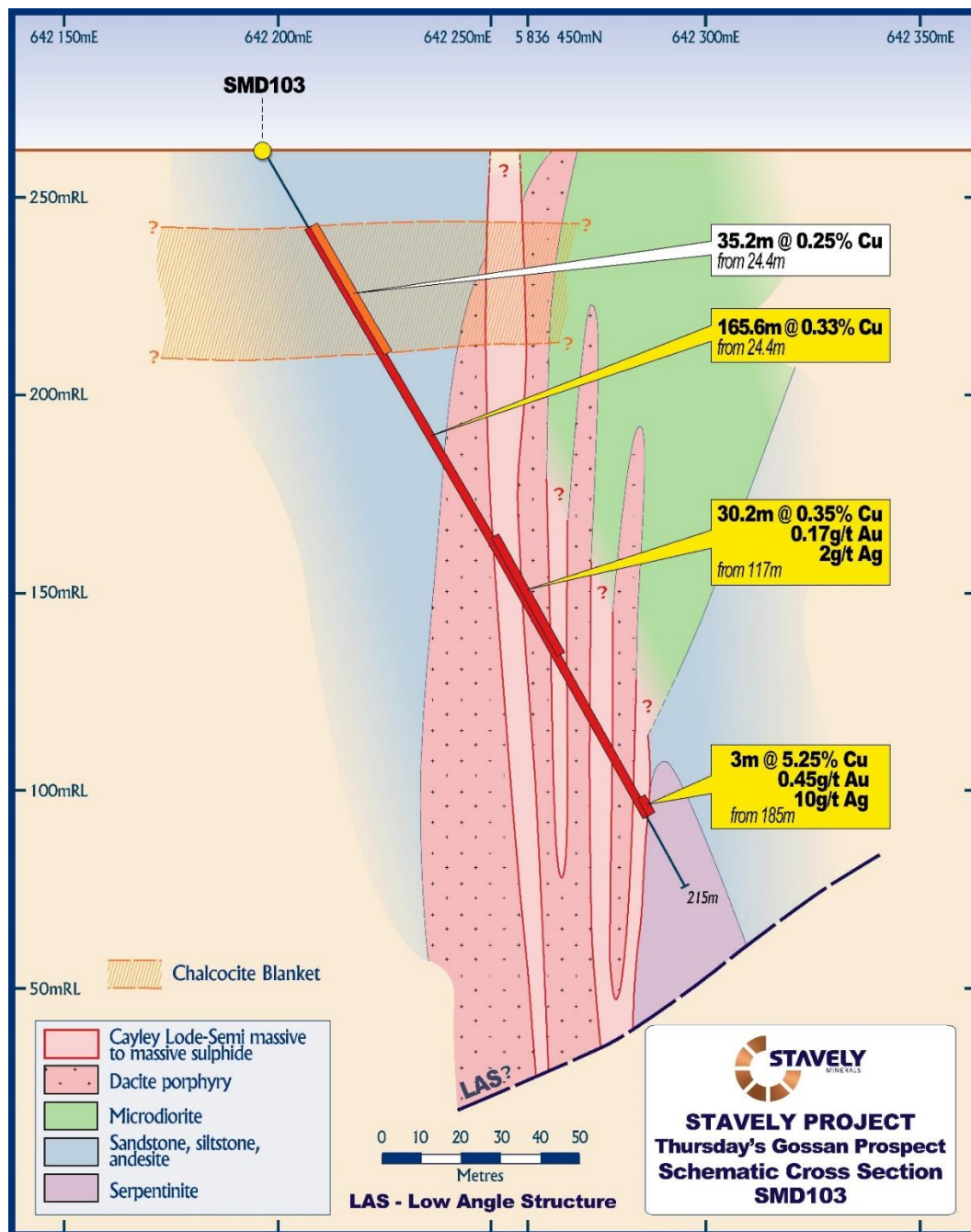
Figure 7. Drill hole SMD103 cross-section.
