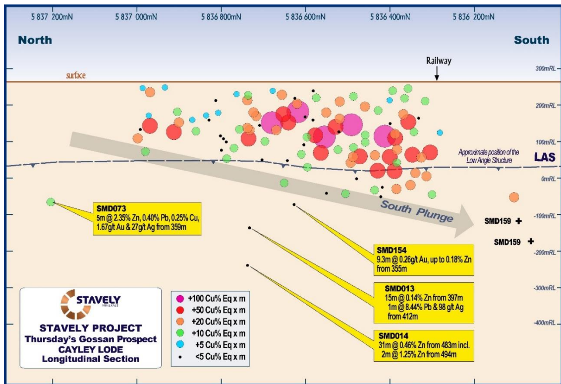
Figure 11. Cayley Lode long section.
