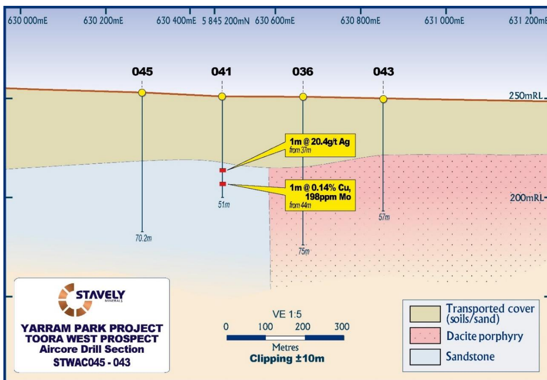
Figure 19. Air-core section including STWAC041.
