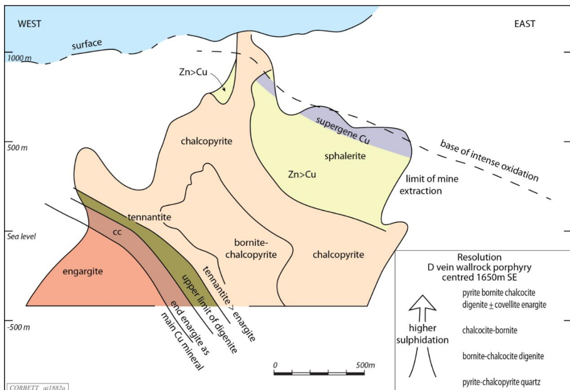
Figure 12. Sulphide zonation of the Magma, Arizona lode-style system.
