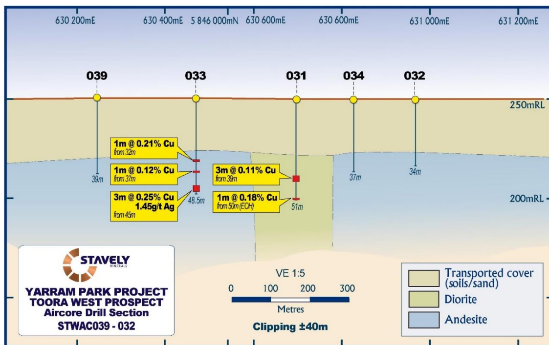
Figure 18. Air-core section including STWAC031-033.
