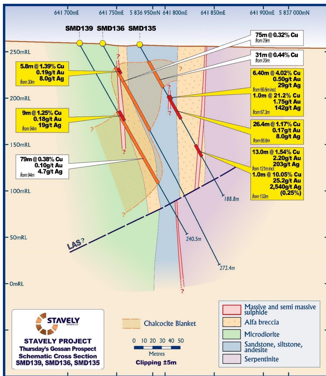
Figure 4. SMD139-SMD136-SMD135 drill section.
