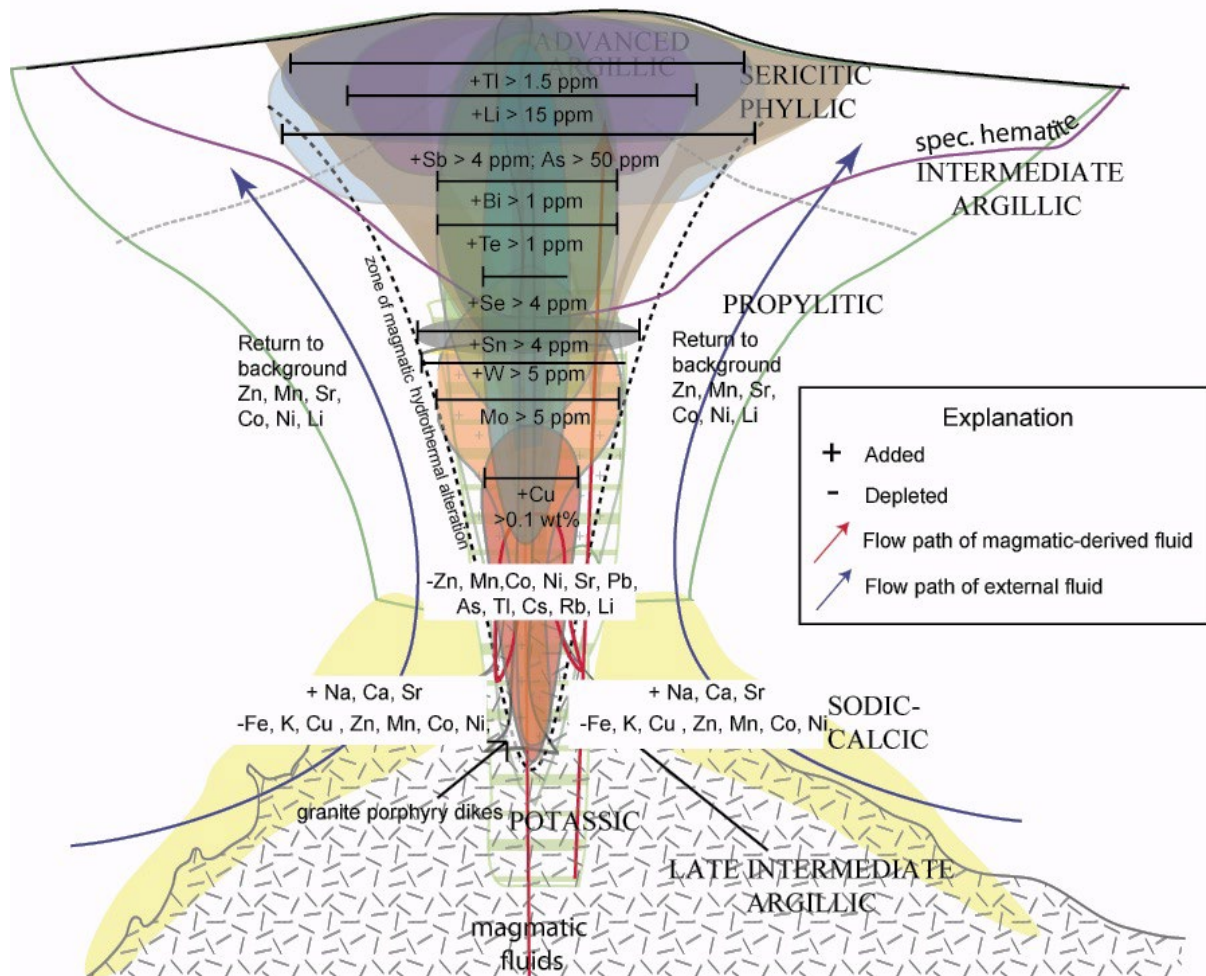
Figure 2. A summary diagram of the Mineral Deposit Research Unit – University of British Columbia generalised model of geochemical and alteration zonation around a porphyry copper-gold deposit (after Cohen, 2011 and Halley et al., 2015). The column of alteration and geochemical zonation depicted may be in the order of 5 kilometres vertically.
