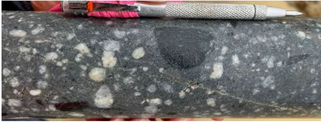
Intensely chlorite altered sandstone xenolith in coarse grained dacite at 279.1m.
