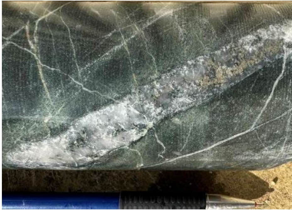
Quartz+carbonate+pyrite vein with rare chalcopyrite. 323.1m.
