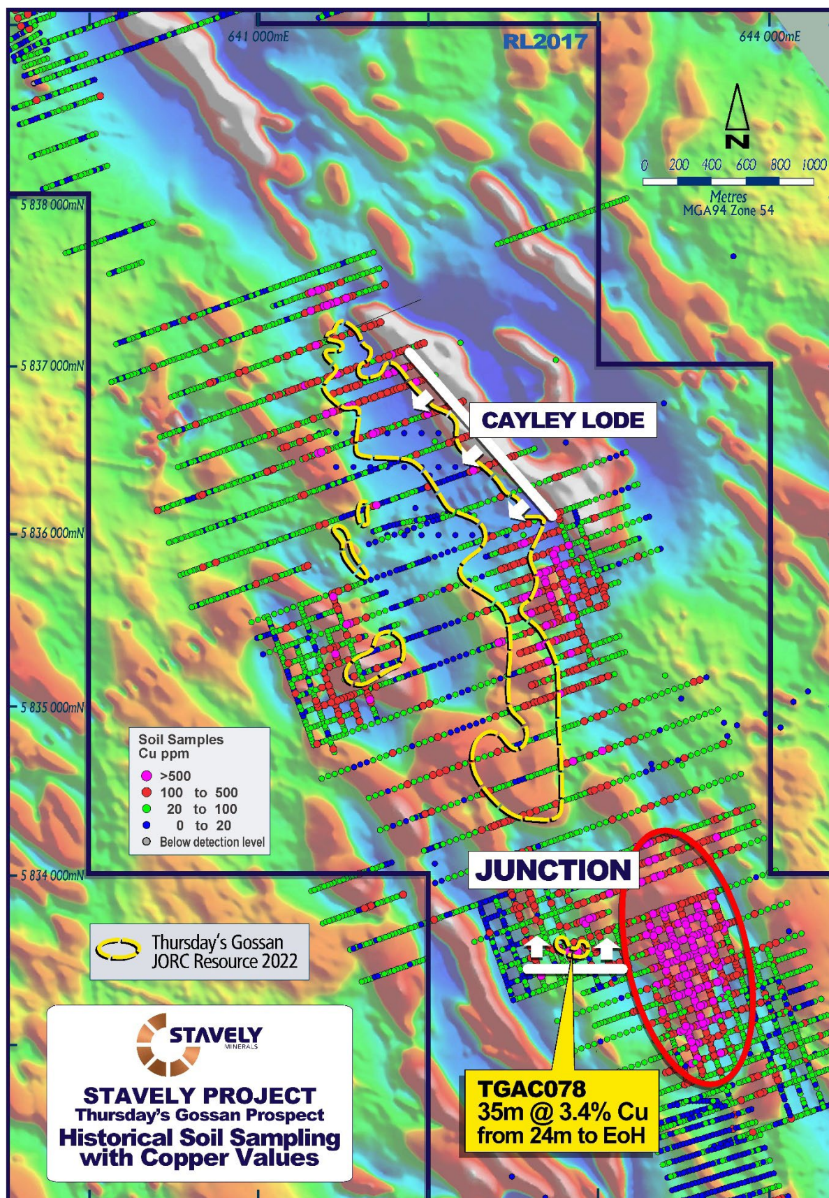
Figure 2. Soil auger copper geochemistry over RTP magnetics showing the location of the Cayley Lodge and the newly interpreted Junction Lodge.
