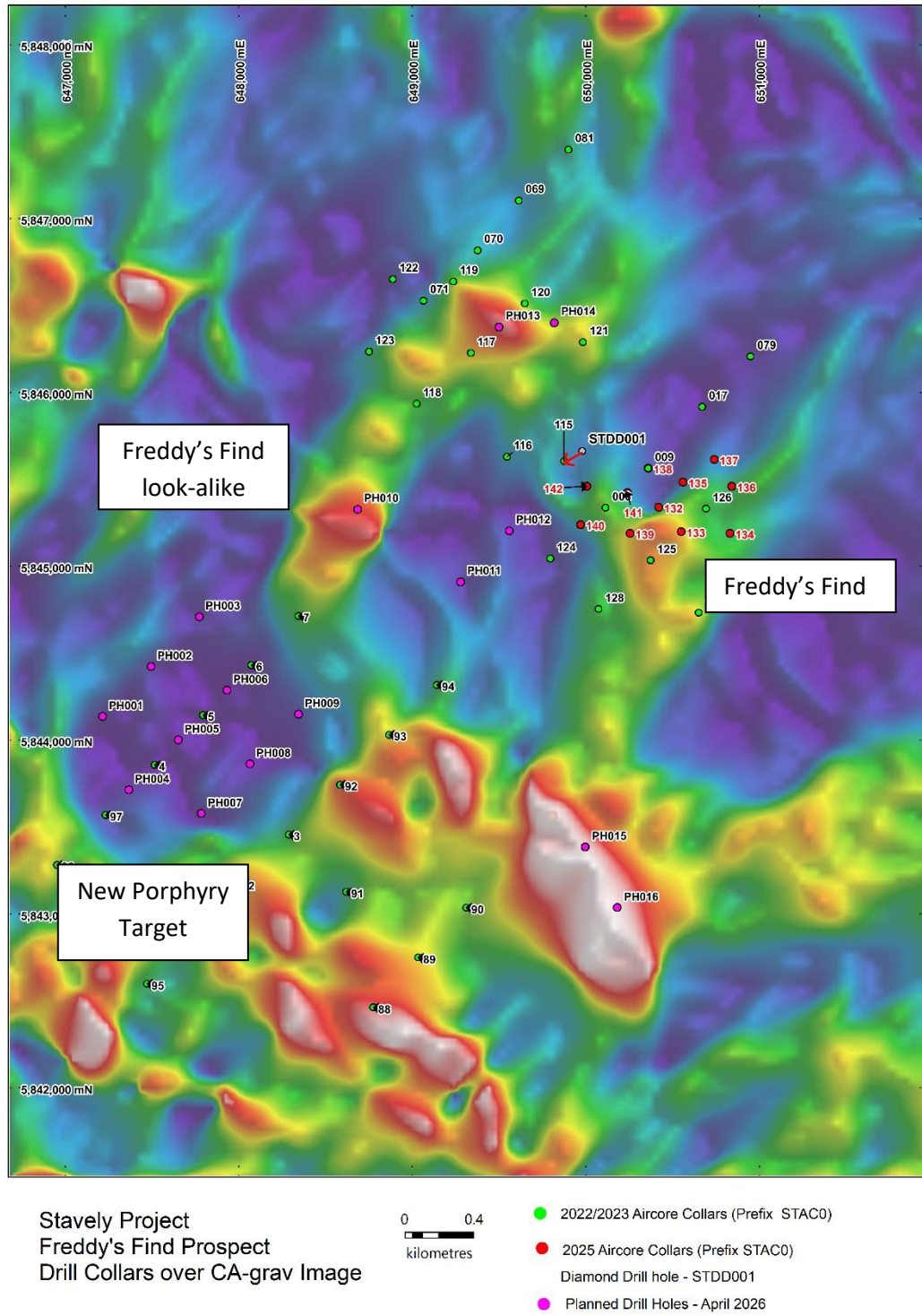
Figure 7. Freddy's Find and New Porphyry Target proposed drilling on gravity image.
