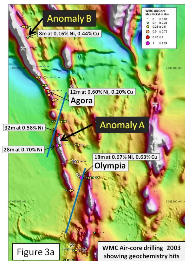
Figure 3: Location of air-core drill holes on magnetic image. 3a) showing the most significant geochemical anomalies including untested Anomaly A & B; 3b) showing the distribution of deep RC & Diamond drill holes
