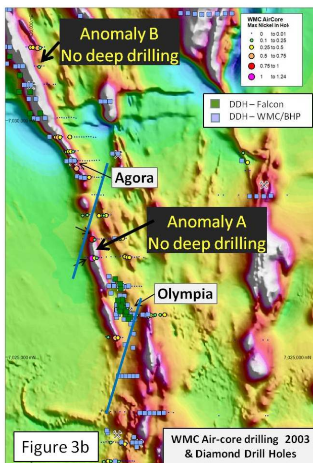
Figure 3: Location of air-core drill holes on magnetic image. 3a) showing the most significant geochemical anomalies including untested Anomaly A & B; 3b) showing the distribution of deep RC & Diamond drill holes
