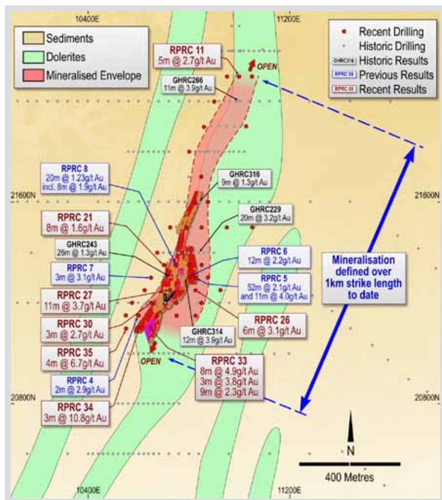
FIGURE 9 – RIPCORD GEOLOGICAL INTERPRETATION
