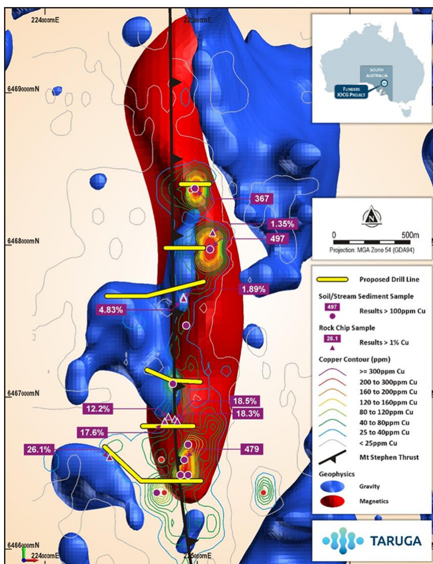
Figure 1: Woolshed/Metabase Geophysical Map showing the Modelled Magnetic Core and Main Gravity Anomalies, Cu in Soil Contours and Rock Chip and Soil Highlights.
