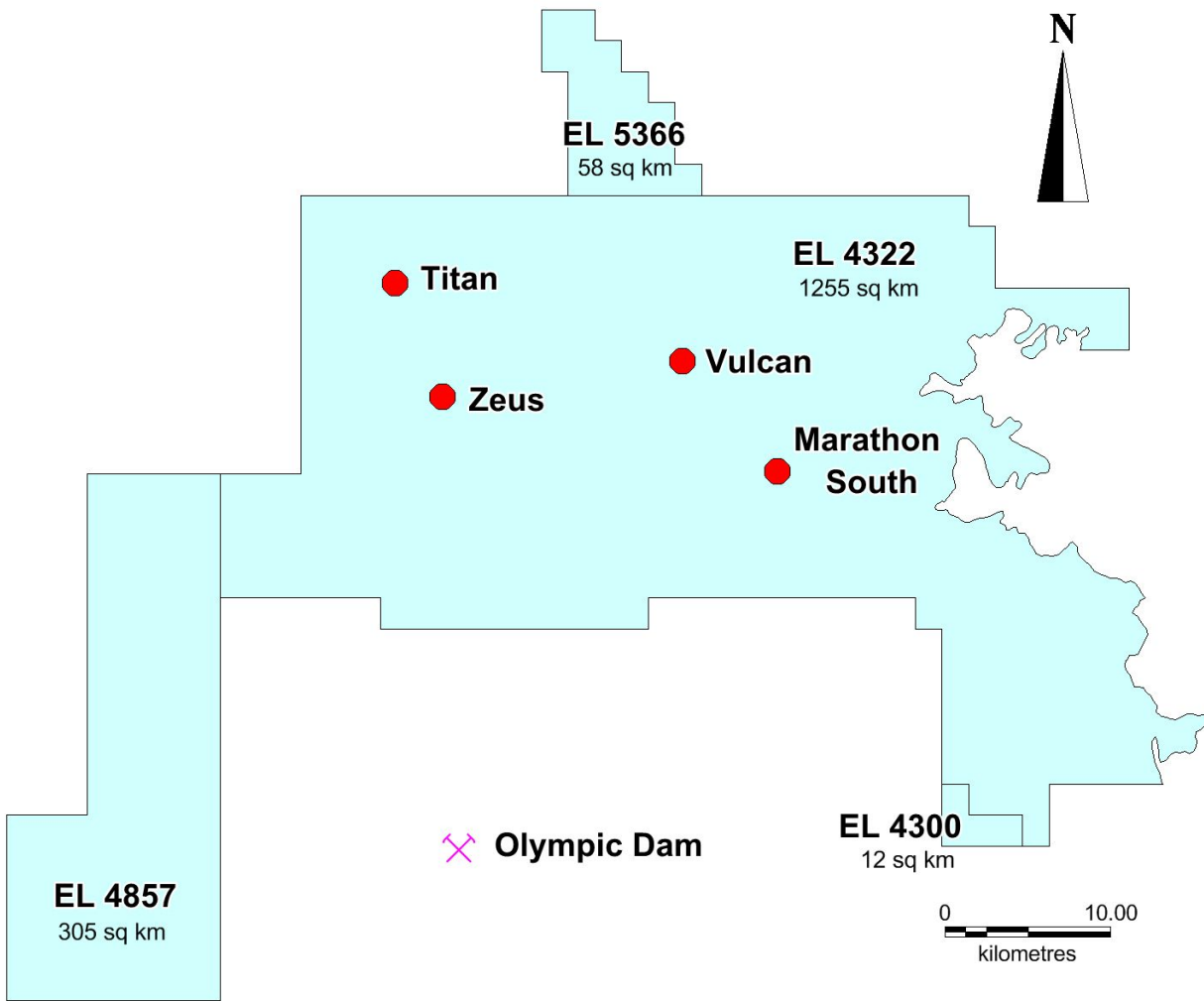
Tasman Resources Ltd, Lake Torrens Project Area Showing Main IOCGU Targets
