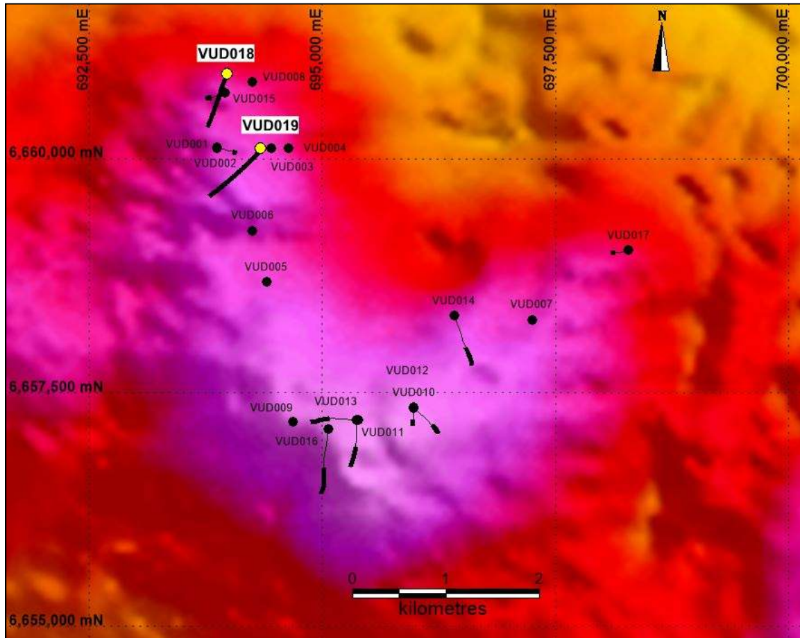
Figure 2: Vulcan Prospect, residual gravity image showing location of VUD 0018 & 0019 and previous Tasman drill holes. The thick black lines on the drill hole traces are the surface projections of basement intercepts (Grid GDA 94, Z53).
