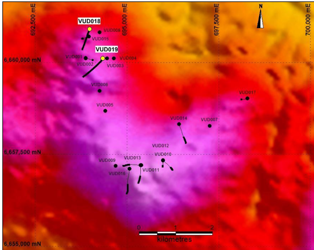
Figure 2: Vulcan Prospect, residual gravity image showing location of VUD0018 & 0019 and previous Tasman drill holes. The thick black lines on the drill hole traces are the surface projections of basement intercepts (Grid GDA 94, Z53).
