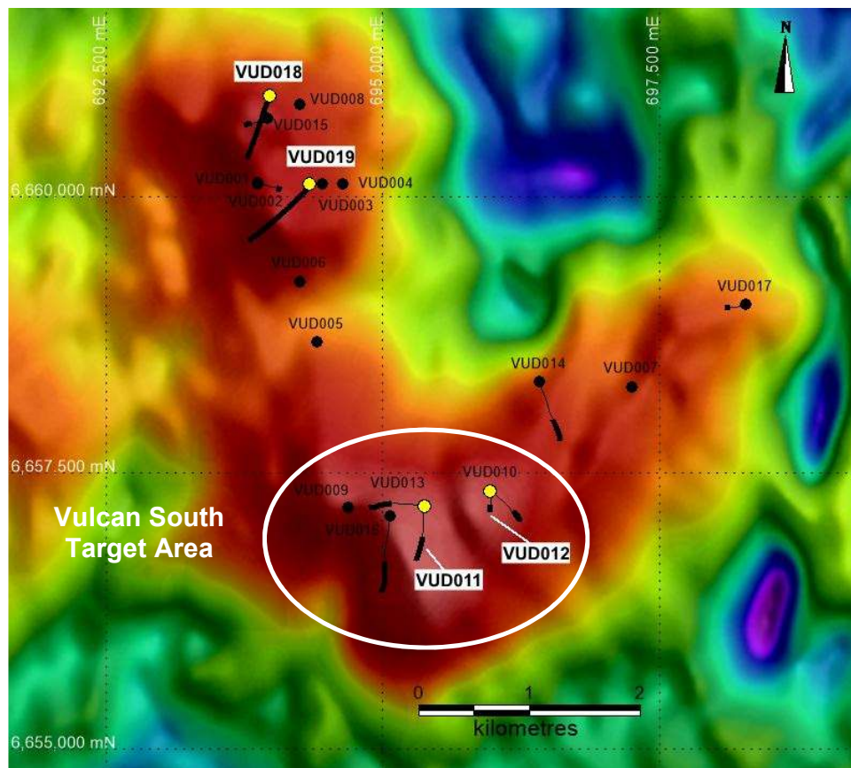
Figure 1: Residual gravity image over the Vulcan Prospect showing the location of Vulcan South, previous Tasman holes VUD011 and 012 and first holes drilled by Fortescue at Vulcan North (VUD018 and 019). The thick black lines on the drill hole traces are the surface projections of basement intercepts (GDA 94, MGA Zone 53).
