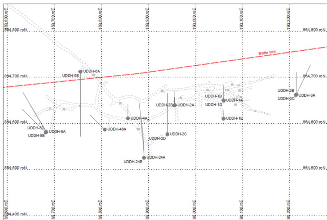
Figure 14: Underground diamond drill hole location map and showing Balite vein which dips steeply south
