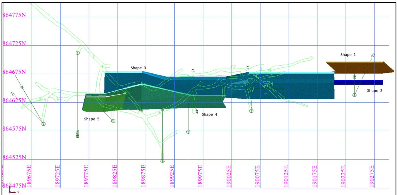
FIGURE 6: Balite Exploration Target showing interpreted lodes (Shape 1 to Shape 5) within the vein system, along with the mine development (green) and diamond drill hole traces (black).
