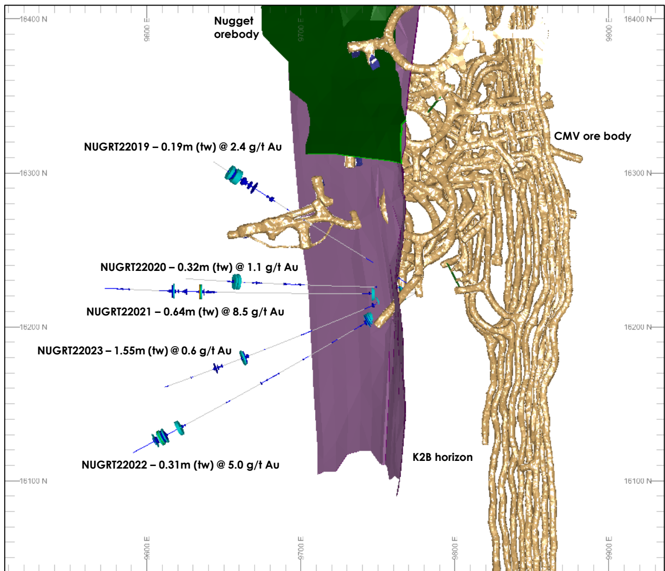
Figure 3: Plan section of results received for Nugget drilling during Q1 FY23
