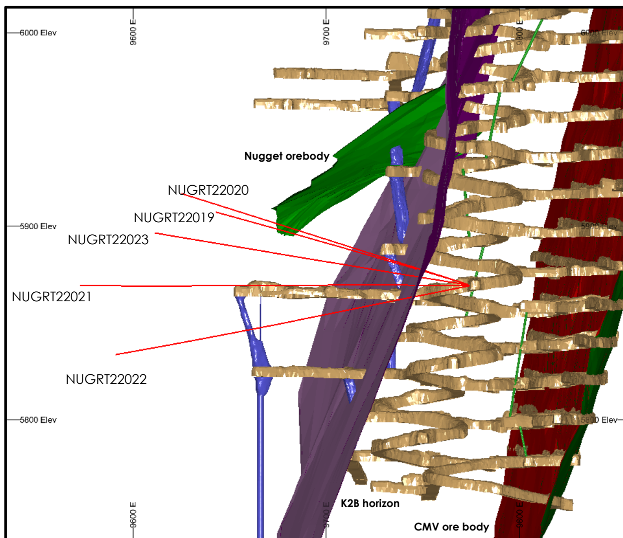
Figure 1: East-west section of Nugget Target Zone drilling undertaken during Q1 FY23.
