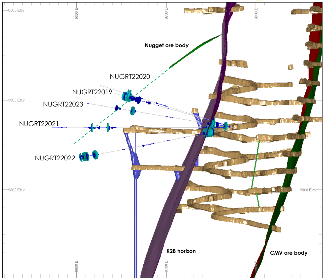
Figure 4: Cross section of results received for the Nugget Drilling Q1, FY23
