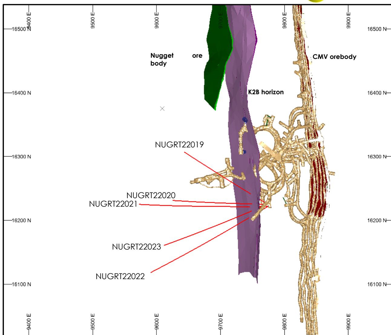
Figure 2: Plan view of Nugget Target Zone drilling undertaken during Q1 FY23.
