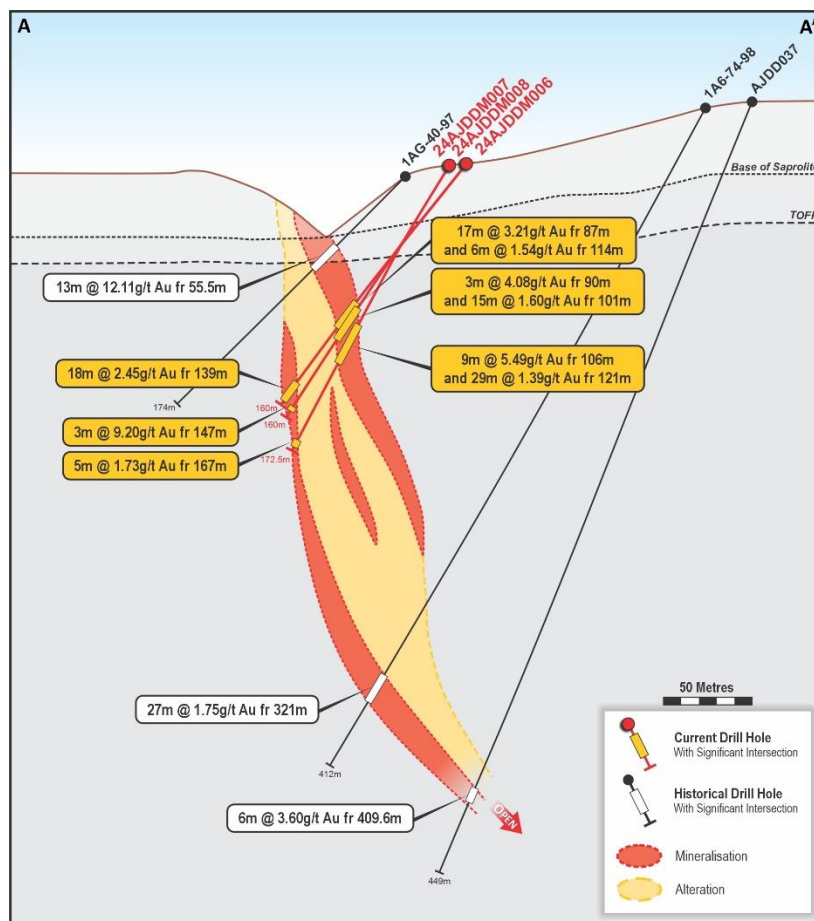
Figure Three | Junction Cross Section (24AJDDM006-008)
