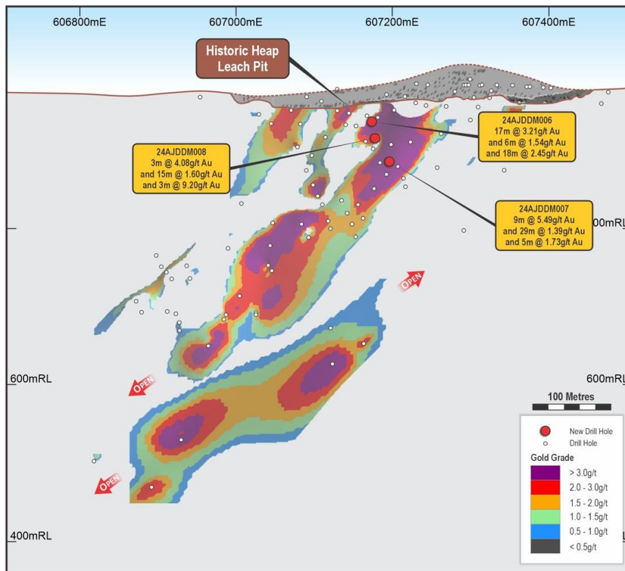
Figure Two | Junction Long Section (looking west showing southerly plunging high grade shoot)
