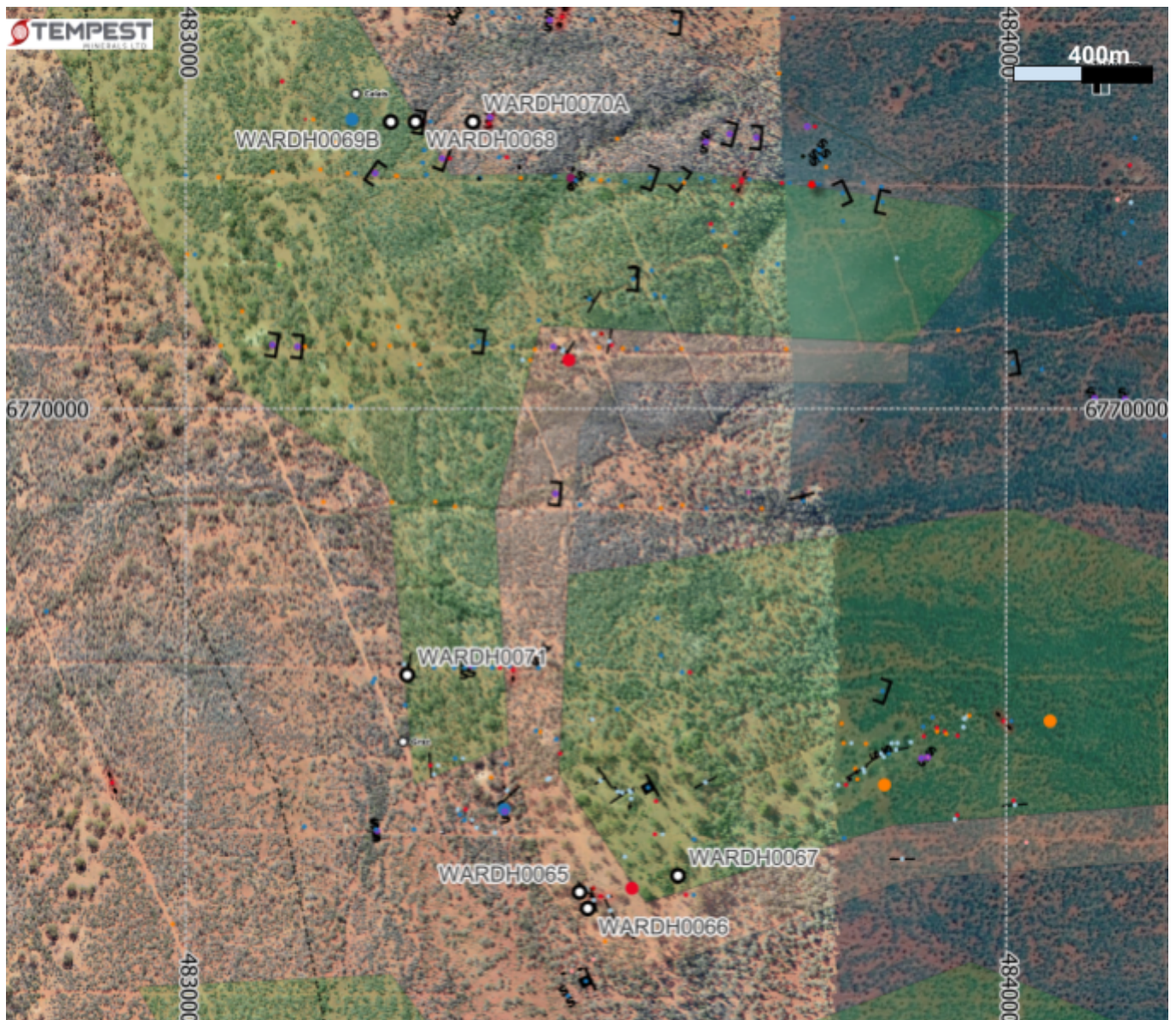
Figure 06: Geological mapping of the drilling area
