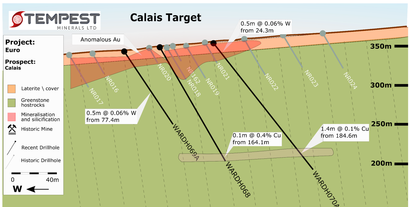
Figure 04: Cross-section through WARDH68-WARDH70A highlighting polymetallic mineralisation
