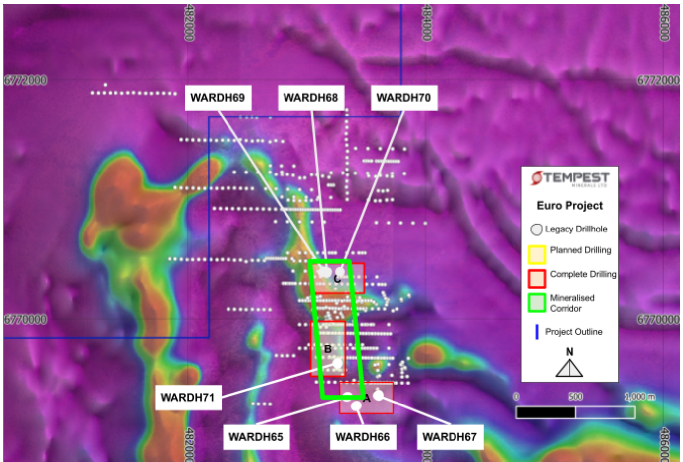
Figure 02: Euro project drilling areas with mineralisation correlated over >1km
