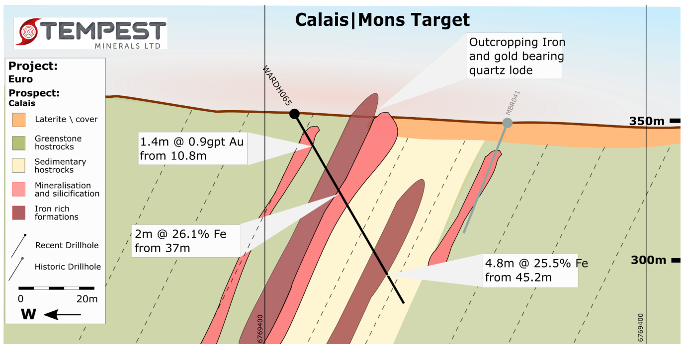
Figure 05: WARDH65 Cross-section showing multiple intercepts of gold and iron mineralisation
