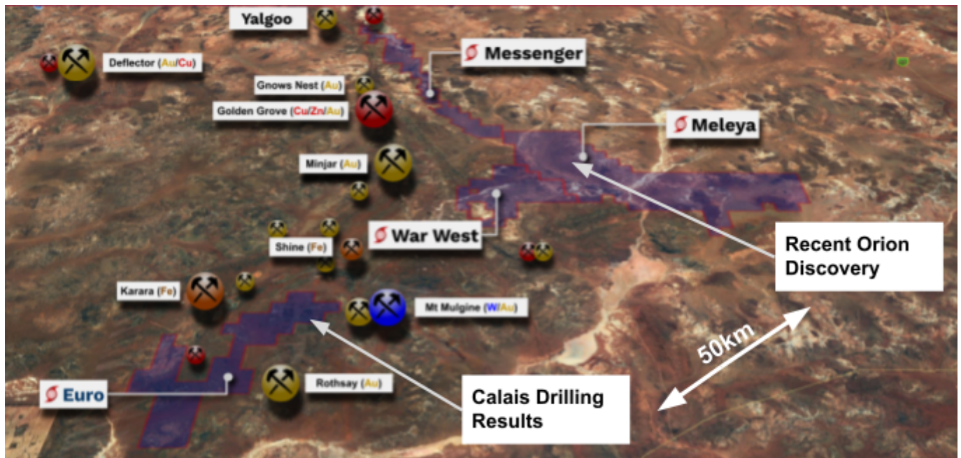
Figure 01: TEM Yalgoo projects regional overview
