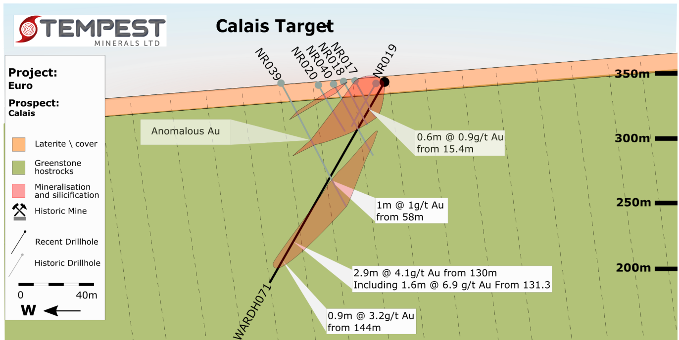
Figure 03: WARDH71 Cross-section showing newly discovered high-grade gold shoot with 1.6m intersection at 6.9g/t Au
