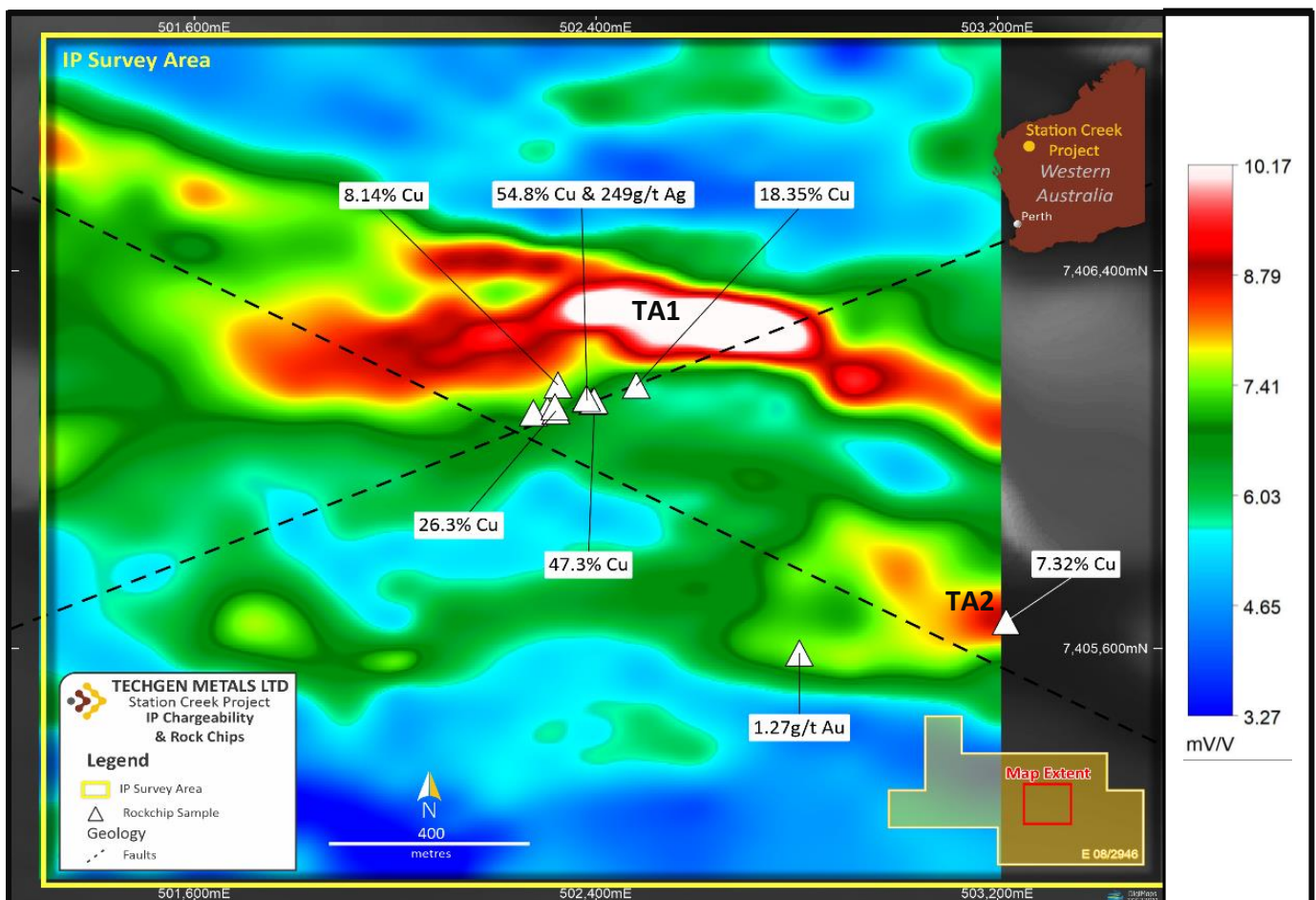
Figure 1: IP chargeability showing the TA1 & TA2 Prospects (white-red area) and interpreted faults.
