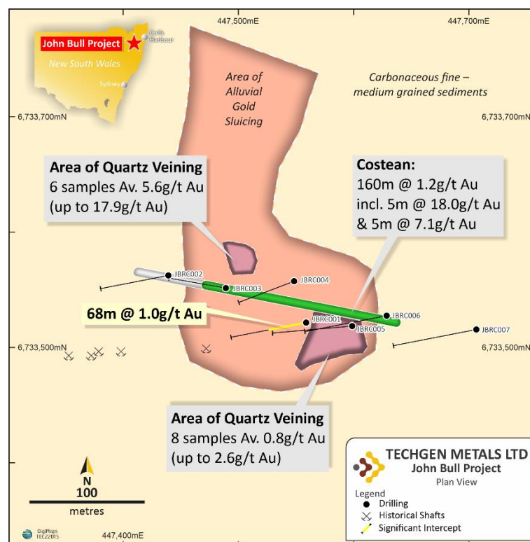
Figure 1: Diagram showing historic shafts, sluicing areas, RC collars, costean and rock chips.
