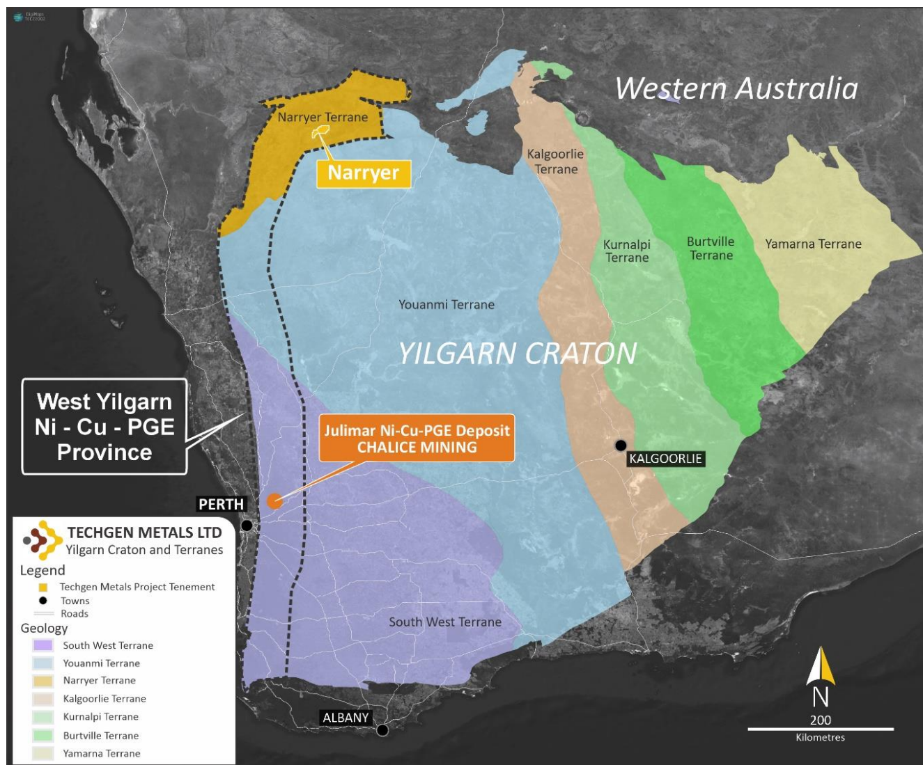
Figure 4: Location of the Narryer Project in the Yilgarn Craton of Western Australia.
