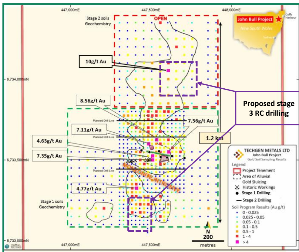
Figure 1: Soil gold geochemistry with planned Stage 3 drilling & completed Stages 1 & 2.
