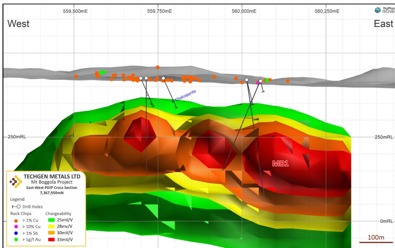
Figure 4: Target MB1 & MB2 East-West IP high chargeability 3D model showing the resistivity (aqua) component.
