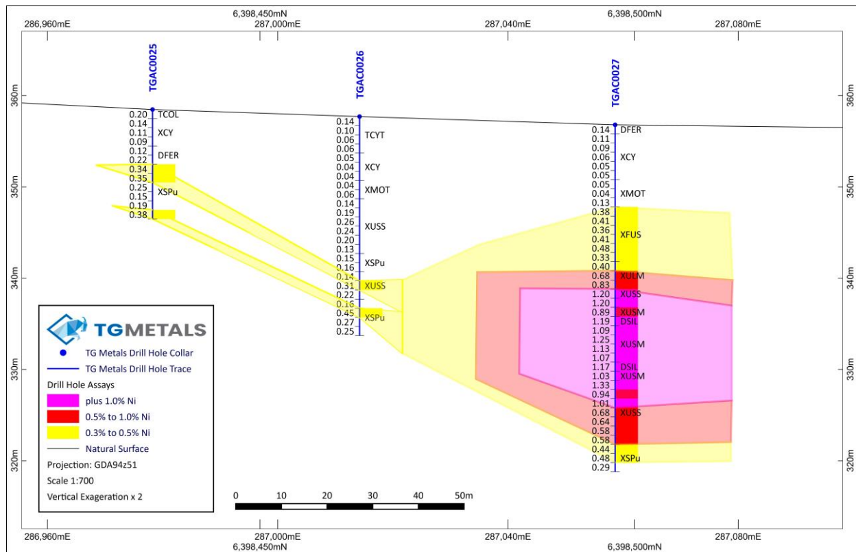
Figure 4 – Thickest intercept cross section TGAC0025 to TGAC0027.
