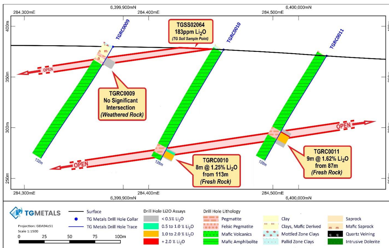
Figure 7 – Cross section TGR0009 to TGR0011 showing lithium pegmatite intercepts and correlation to elevated Li 2 O soil sample grades
