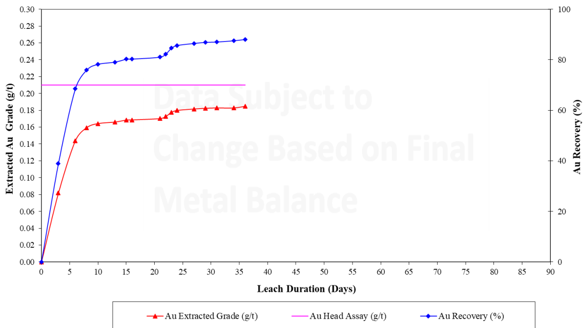
Figure 6 - Leaching Times for Column Two Leach Tests
