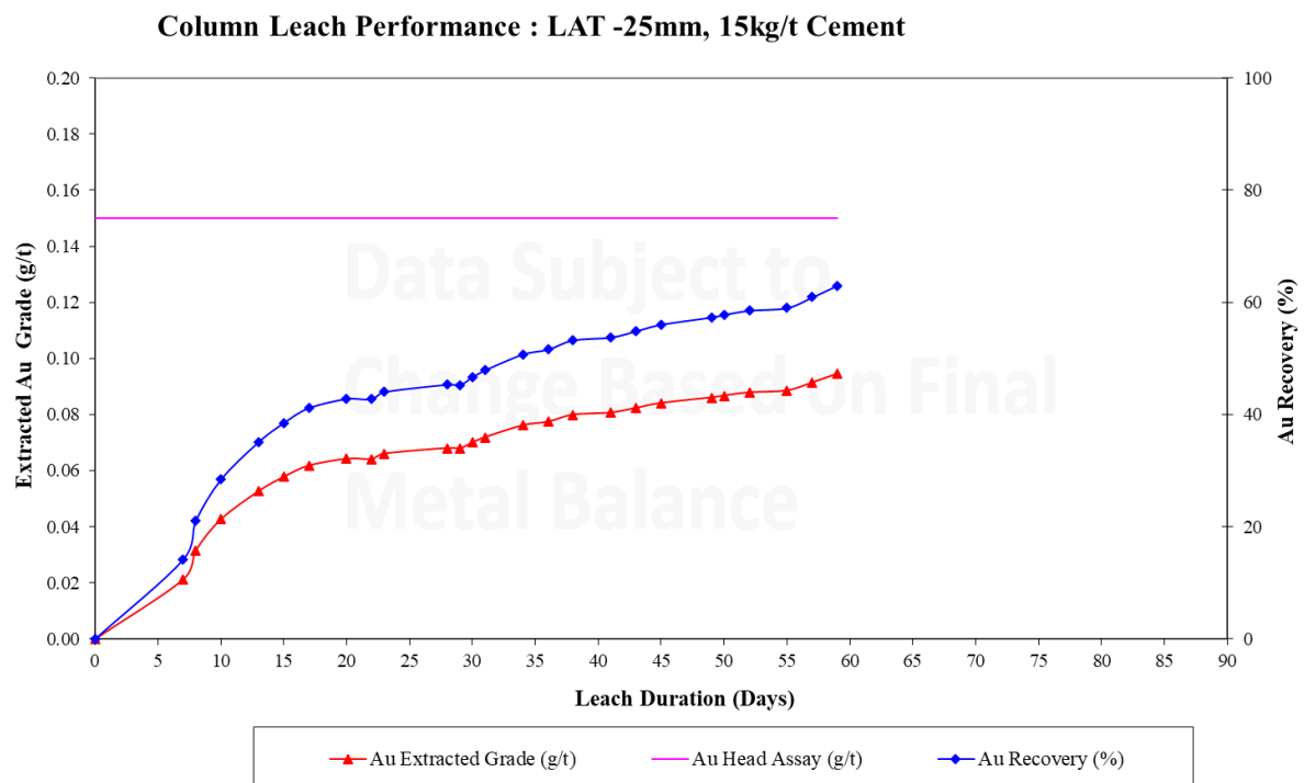
Figure 2 - Leaching Times for Column One Leach Tests
