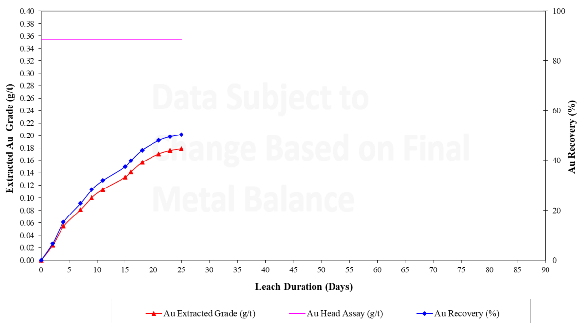
Figure 4 - Leaching Times for Column Three Leach Tests
