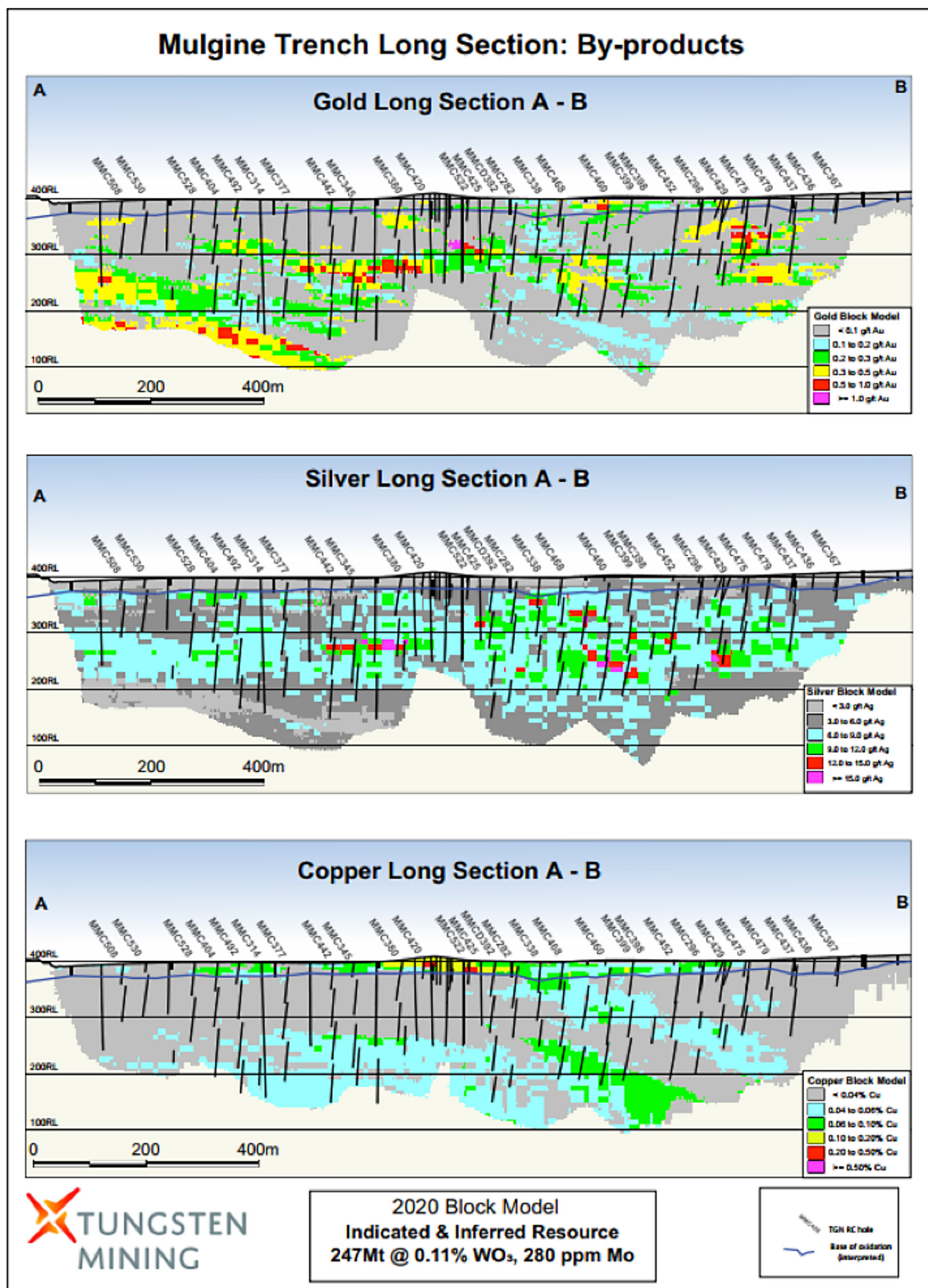
Figure 8 – Long section through Mulgine Trench showing gold (top), silver (middle) and copper (bottom) grades for the May 2020 Mineral Resource Block Model. Stronger by-product mineralisation tends to be associated with the Lower Tungsten-Molybdenum domain.
