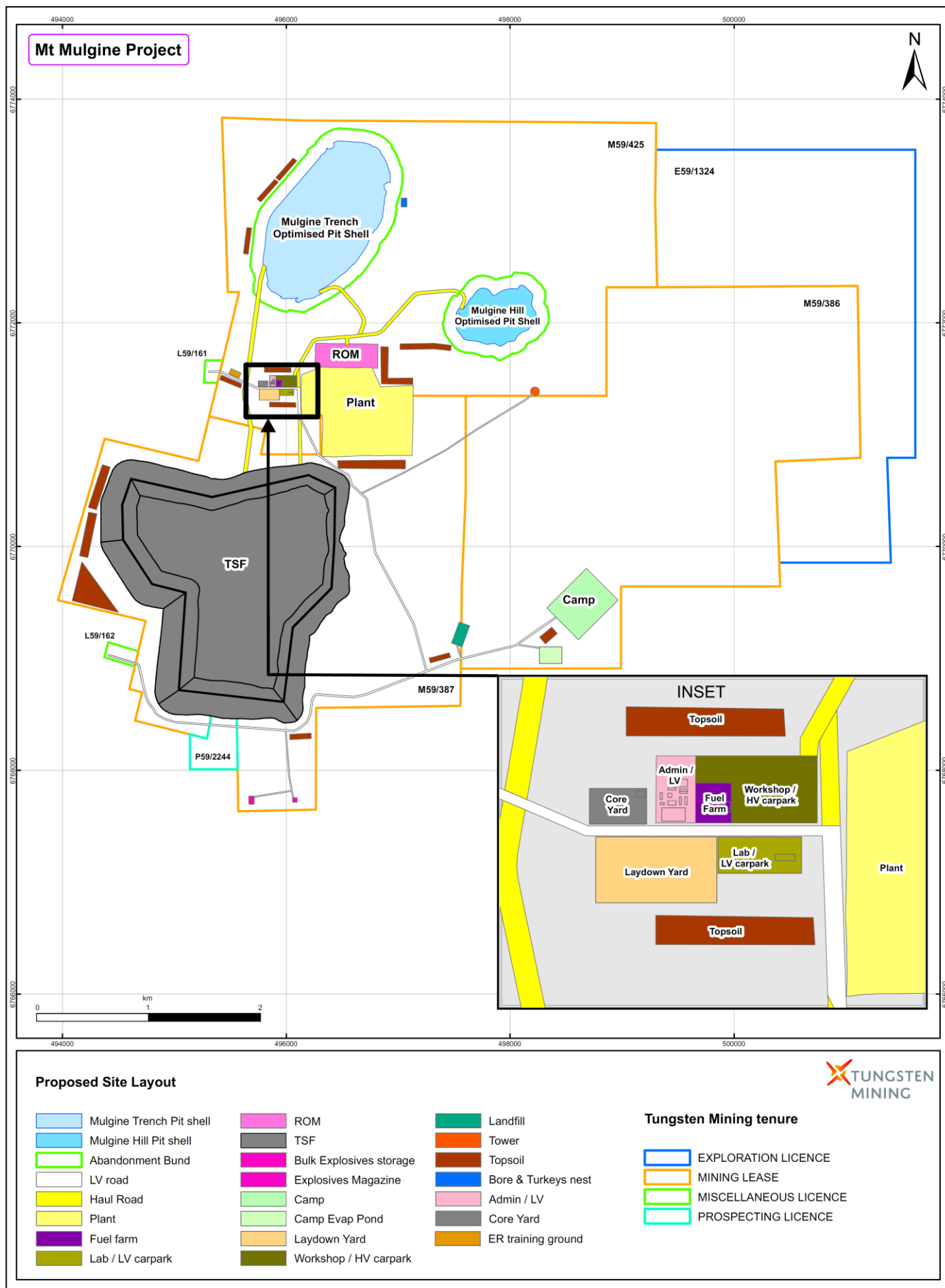
Figure 3 – Project Layout
