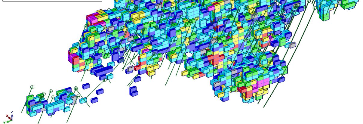
Figure 4-2: Watershed Mineral Resources WO 3 Grades (Oblique View)
