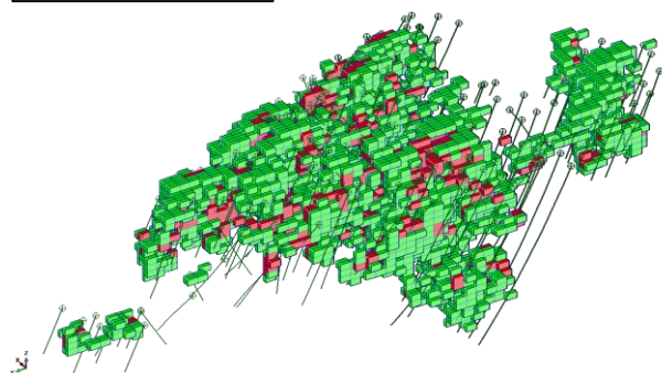
Figure 4-1: Watershed Mineral Resource Category (Oblique View)
