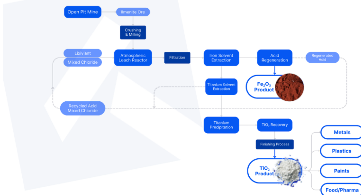
Figure 1: Simplified RCL \text{TiO}_2 flowsheet and layout – how we process the feed
