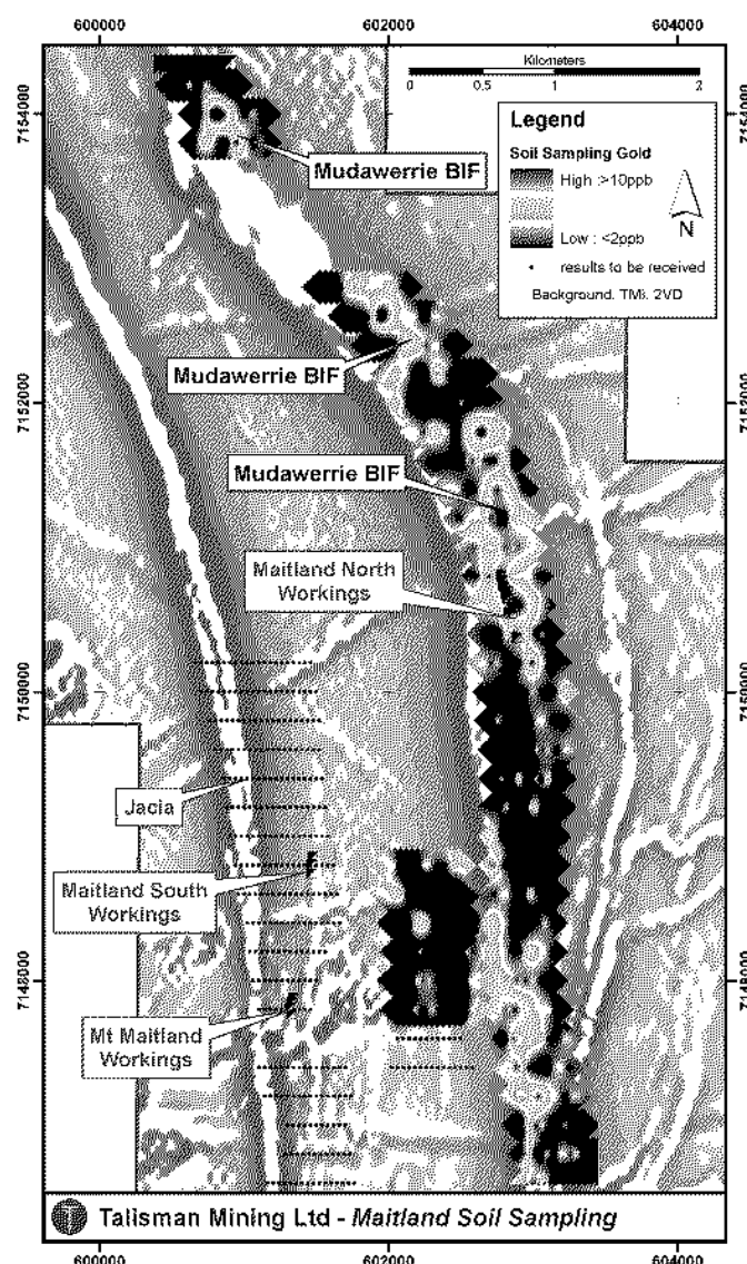
Figure 3: Maitland Project – Soil Geochemistry
