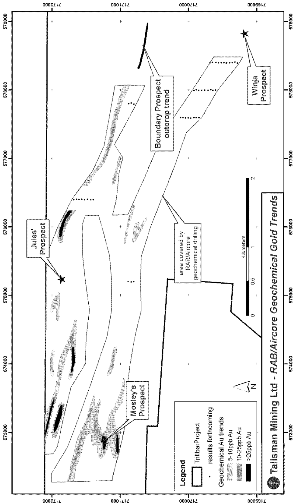
Figure 2: Trillbar Project – RAB / Aircore Saprolite Geochemistry
