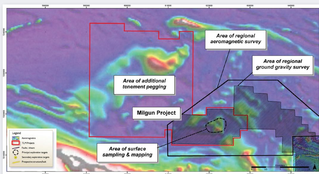
FIGURE 5 – Milgun Project Geology and Airborne Magnetism
