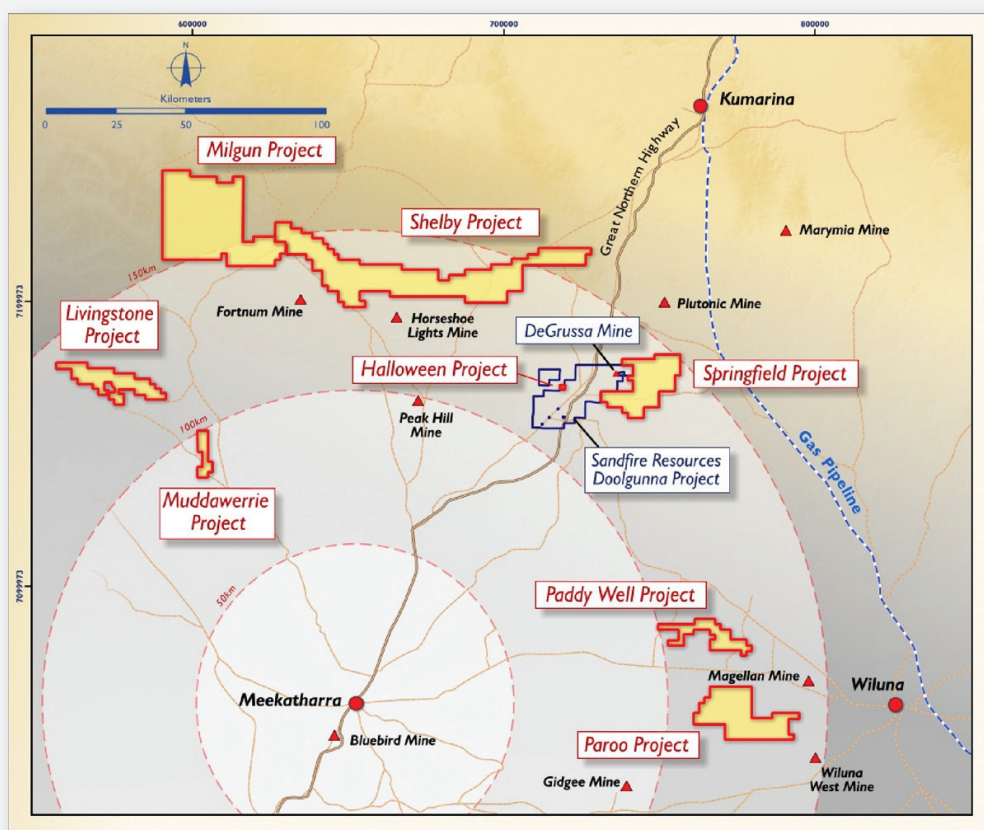
FIGURE 1 - Talisman Mining Project Locations
