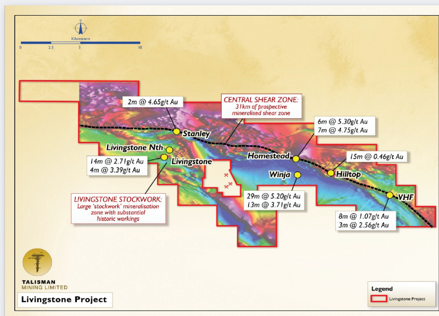
FIGURE 7 – Livingstone Gold Project
