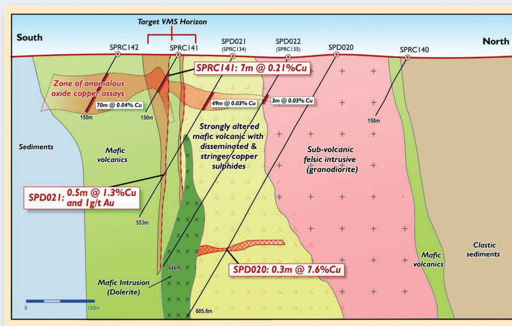
FIGURE 2 – Monty Prospect Interpreted Section (743600mE)
