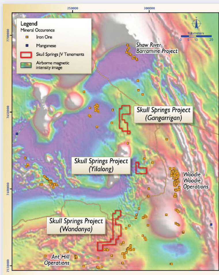
FIGURE 8 – Skull Springs Tenements
