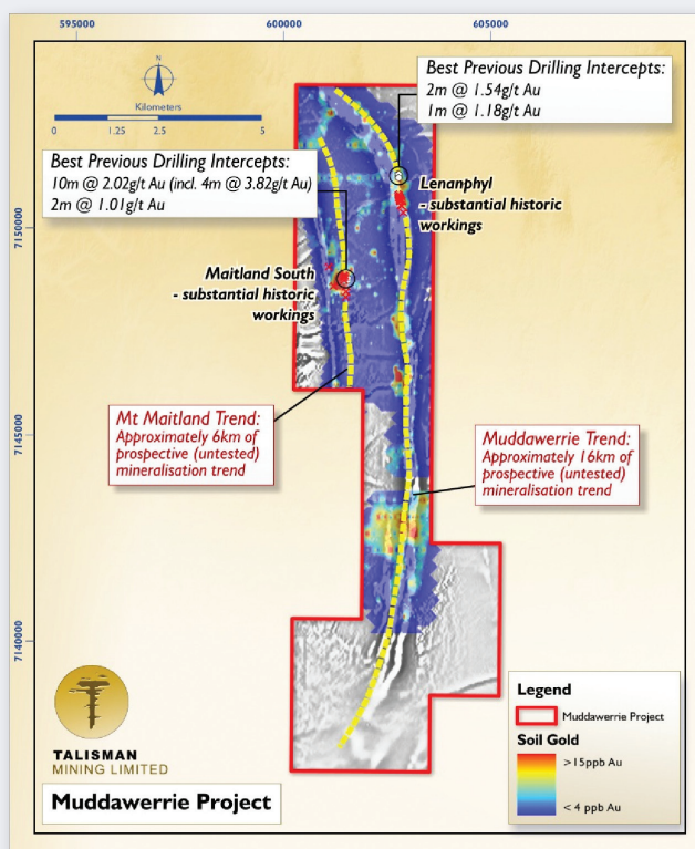
FIGURE 6 – Muddawerrie Gold Project
