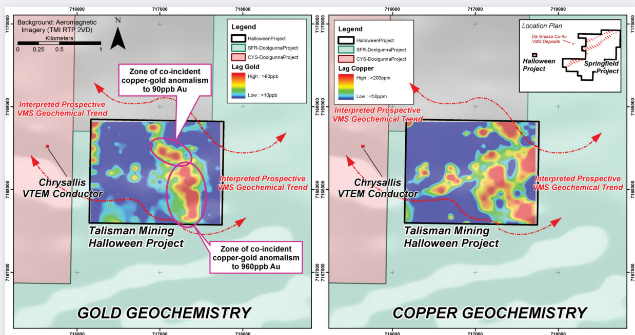
FIGURE 3 – Halloween Project Gold and Copper Geochemistry
