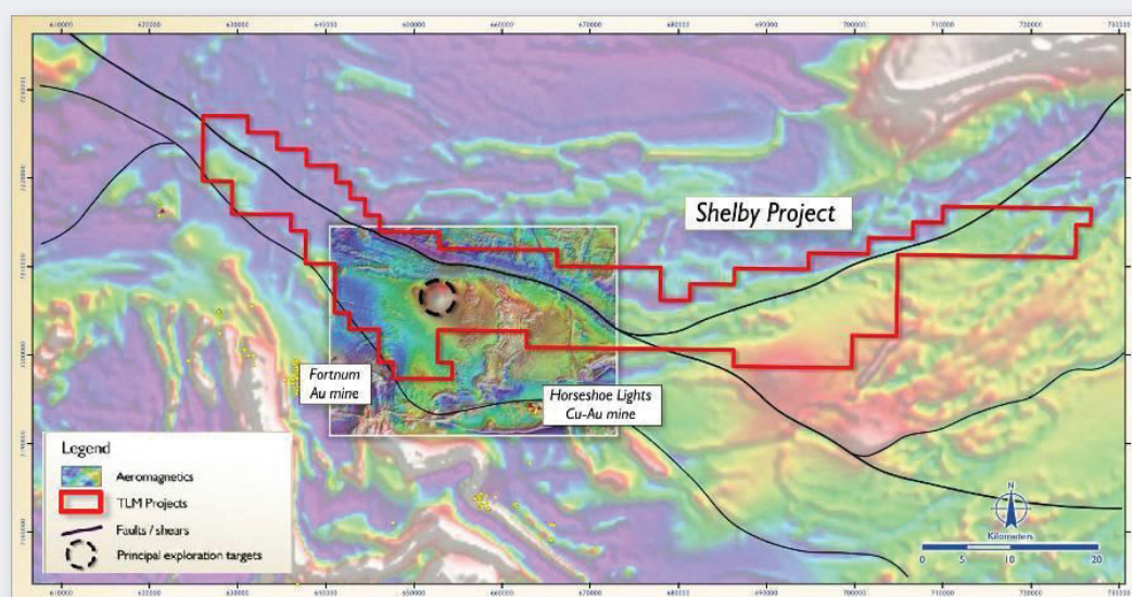
FIGURE 4 – Shelby Project Airborne Magnetics
