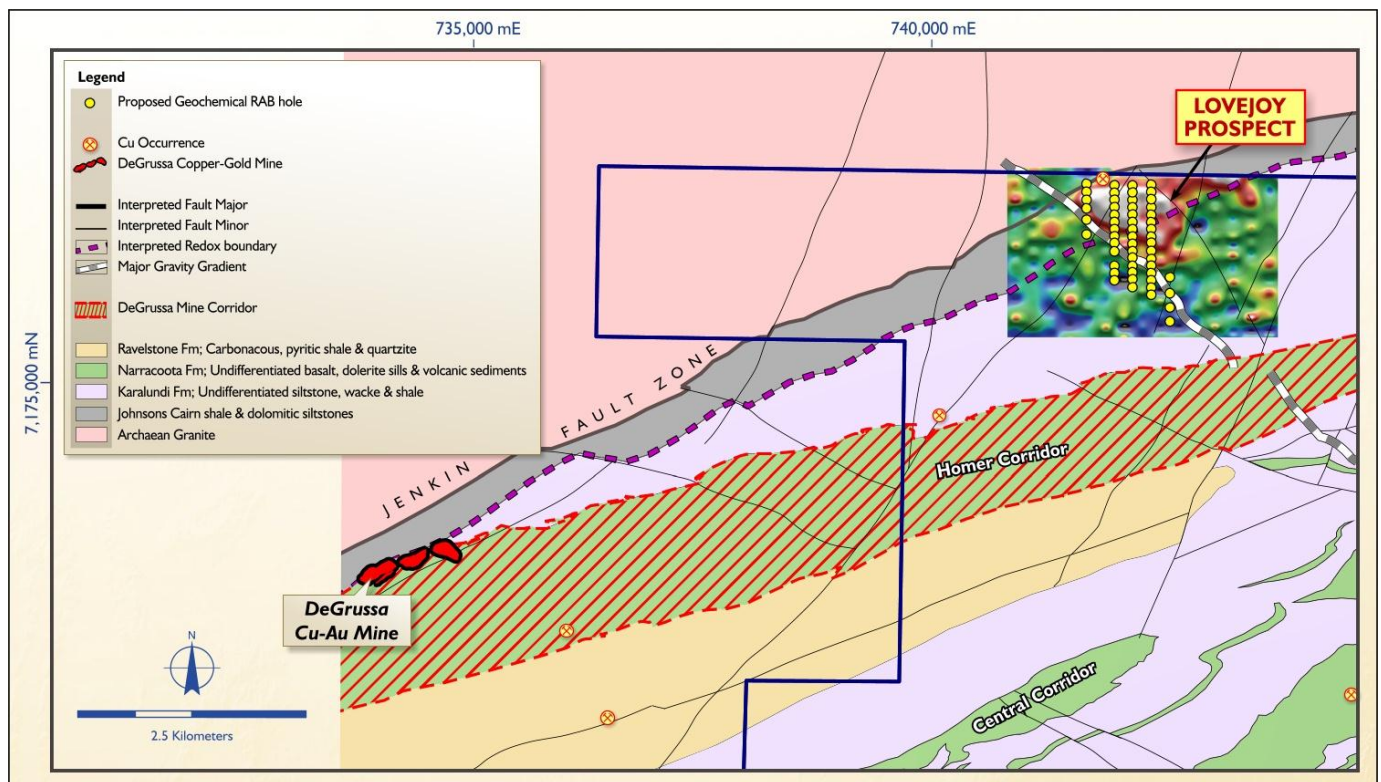
Figure 2 – Springfield geology map showing planned geochemical RAB drilling over Lovejoy MLEM target associated with an interpreted major redox front and NW trending gravity structure
