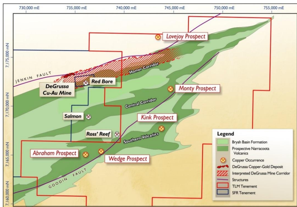
Figure 1 – Springfield Project, simplified geology showing Prospect locations
