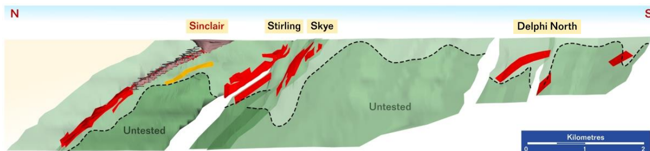
Figure 5: Oblique projection of the Sinclair Ultramafic trend
