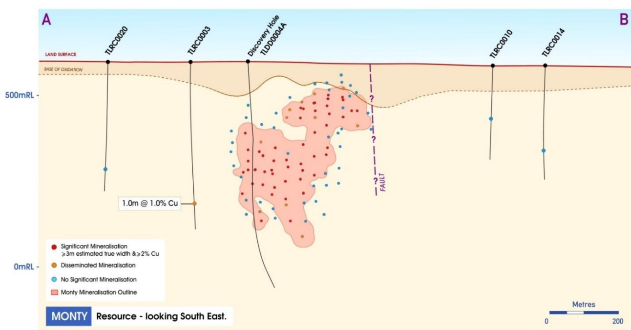
Figure 2: Stylised vertical longitudinal projection by Talisman showing Monty Resource outline and all RC and diamond holes intersecting the interpreted host horizon
